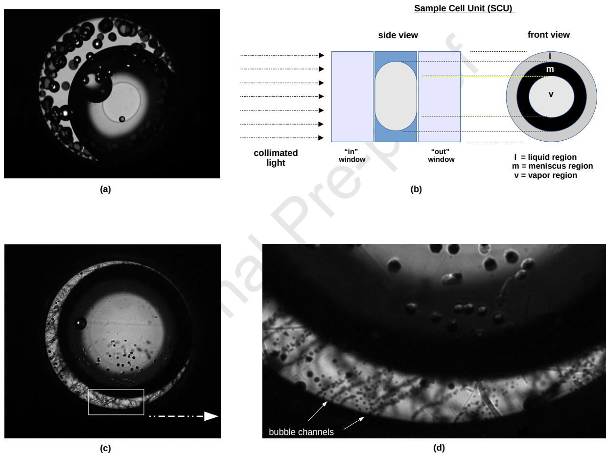
Figure 4: Images showing comparison of incipient boiling of (a) pure water and (c) Na 2 SO 4 (aq) 5%-w and (d) the enlarged inset to show the vapor channels comprising small vapor bubbles moving radially inward from the heated surface to the liquid-vapor meniscus. The schematic (b) provides an explanation of the view that is presented in the images.
