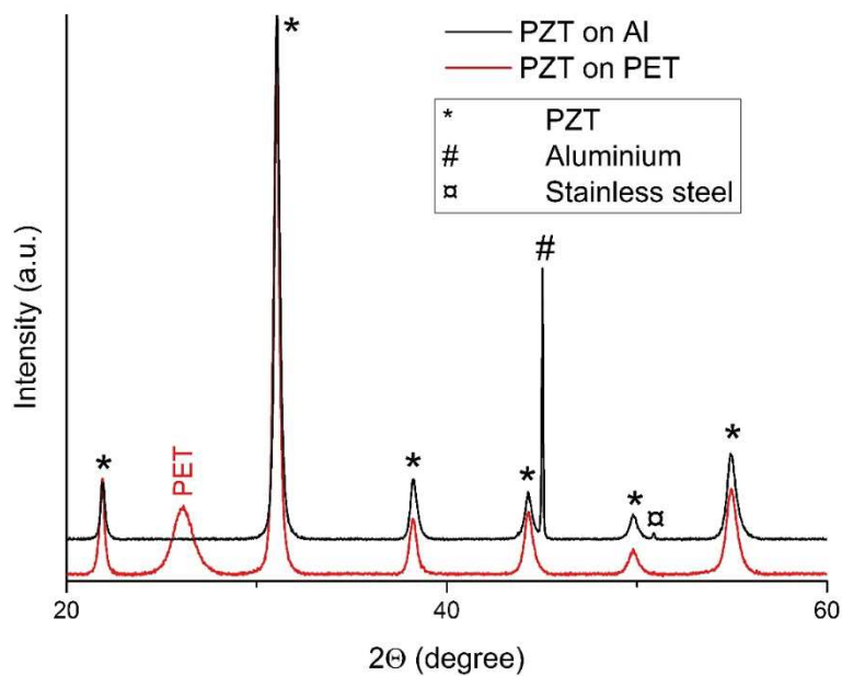
Fig 8 : XRD patterns of PZT before and after transfer from aluminium substrate to PET substrate.
