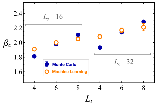
Figure 13: The critical coupling constant \beta_c of compact electrodynamics at various lattices L_s^2 \times L_t . The full symbols: the Monte-Carlo results obtained from the original gauge-field configurations. The open symbols: the prediction of the neural network based on monopole configurations only.
