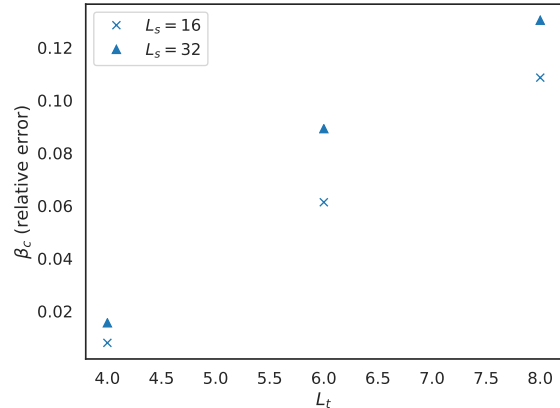
Figure 12: Relative errors in terms of L_t and L_s for \beta_c computed from \langle p(\phi) \rangle .
