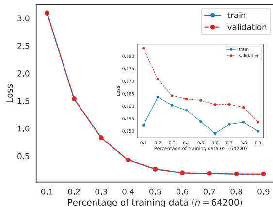
Figure 4: Learning curve (evolution of losses for the training and validation sets of different sizes). The inset: the learning curve without regularization.
