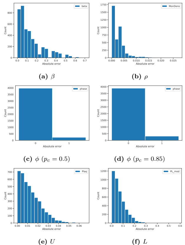
Figure 6: Comparison of absolute errors on the predicted distributions.
