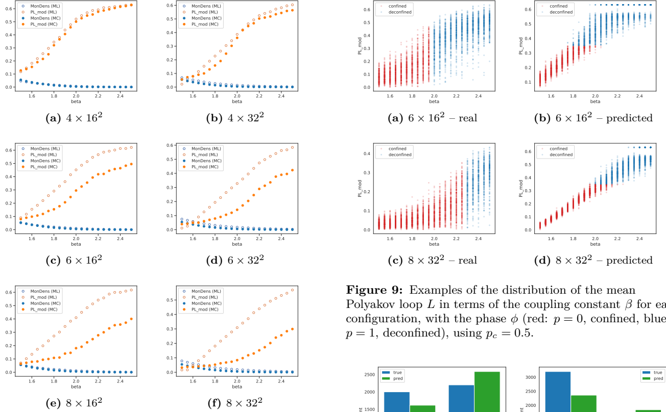
Figure 8: The monopole density \langle \rho \rangle and the Polyakov loop \langle L \rangle in terms of \beta . The filled symbols show the actual quantities calculated with the help of Monte-Carlo (MC) technique and the open symbols are the predictions based on the machine learning (ML) of the monopole configurations.
