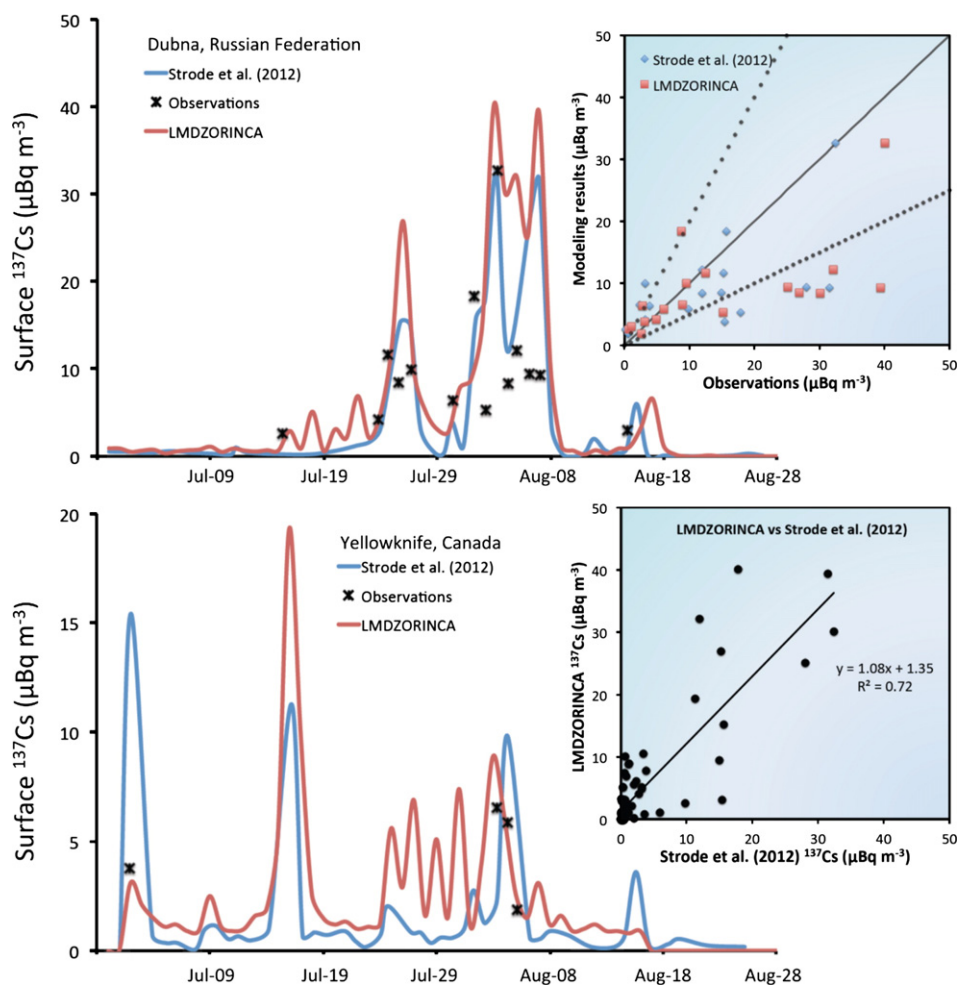
Fig. 7. Comparison of the LMDZORINCA model was used to simulate fire scenarios with the calculations of Strode et al. (2012) and CTBTO observations for the original forest fires of 2010. Our model computed surface concentrations of ^{137}\text{Cs} very efficient recording the arrival times of the plume to each station and the main peaks as well, while high consistency was achieved with observations and with the modeling results reported by Strode et al. (2012).
