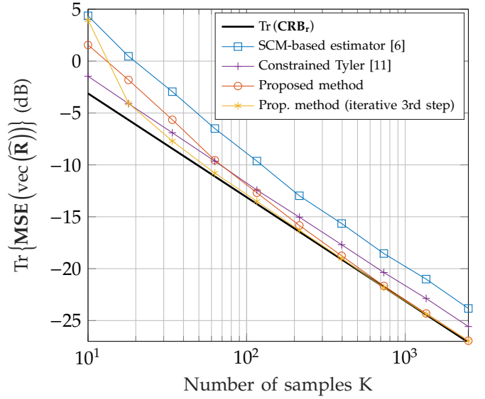
Figure 1. Efficiency simulation
