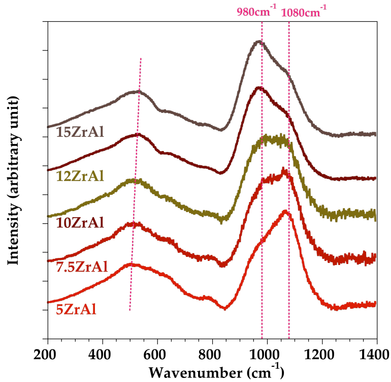
Fig. 10. Raman spectra acquired on glasses. Some spectra have been displaced for clarity. Lines indicate the shift of the band at \sim 500\text{ cm}^{-1} and the position of the bands at 980\text{ cm}^{-1} and 1080\text{ cm}^{-1} .
