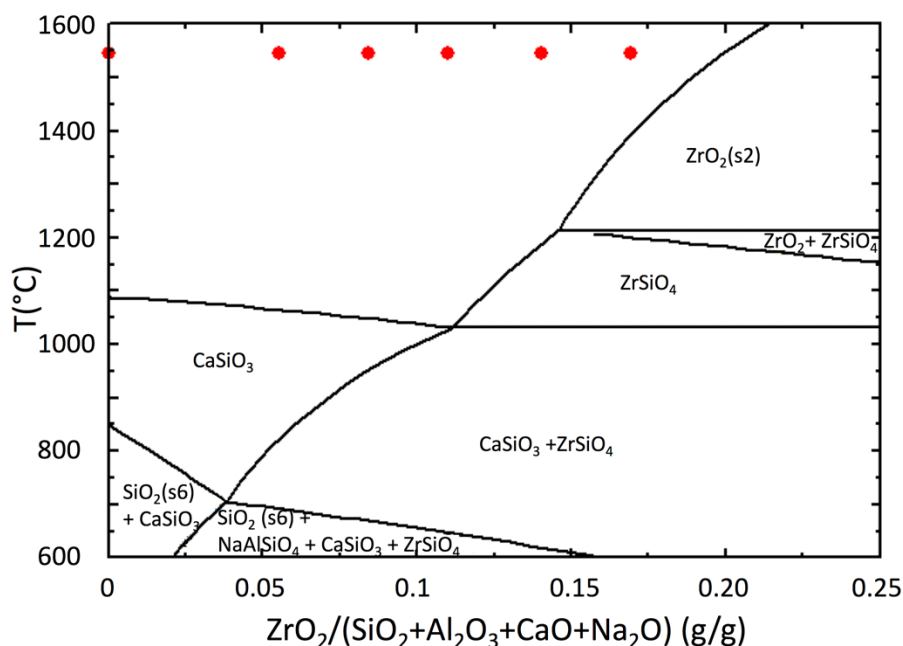
Fig. 1. Phase diagram in a \text{Na}_2\text{O-CaO-Al}_2\text{O}_3\text{-SiO}_2\text{-ZrO}_2 system with increasing \text{ZrO}_2 content (wt%). \text{ZrO}_2(\text{s}2)=\text{t-ZrO}_2 , \text{ZrO}_2=\text{m-ZrO}_2 , \text{SiO}_2(\text{S}6)=\text{cristobalite} . The red points correspond to the \text{ZrO}_2 content
