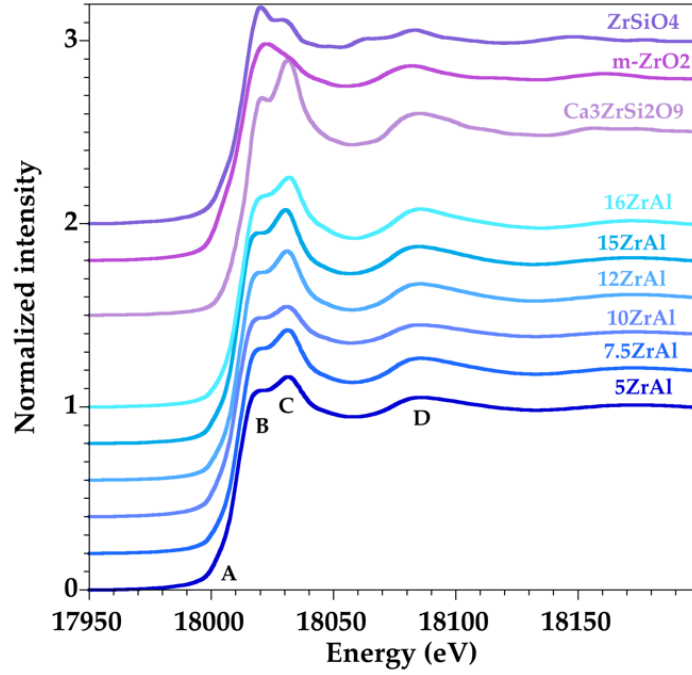
Fig. 7. XANES spectra at Zr K-edge for crystalline references and glasses.
