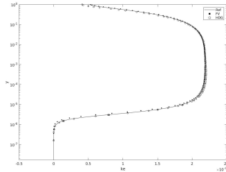
Fig. 9: k at Re = 2 \times 10^8 with 120 DOFs at y^+ = 0.29
