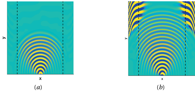
Figure 2. Snapshots of the electric field component E_1(t, x, y, 0) at (a) t = 2.5 , (b) t = 4 for a medium with diagonal anisotropy defined by \varepsilon_1 = 10, \varepsilon_2 = 20, \varepsilon_3 = 1 .
