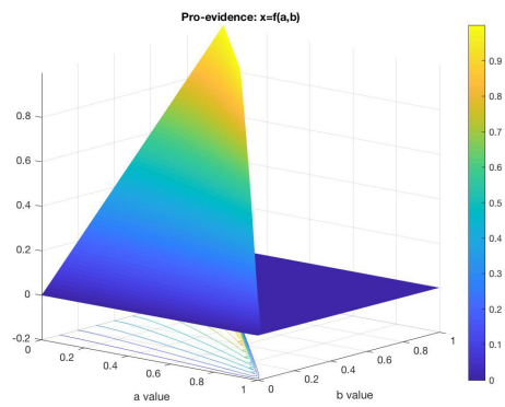
Figure 2: Plot of x = f(a, b) pro-evidence surface.
