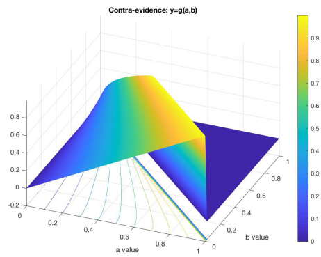
Figure 3: Plot of y = g(a, b) contra-evidence surface.
