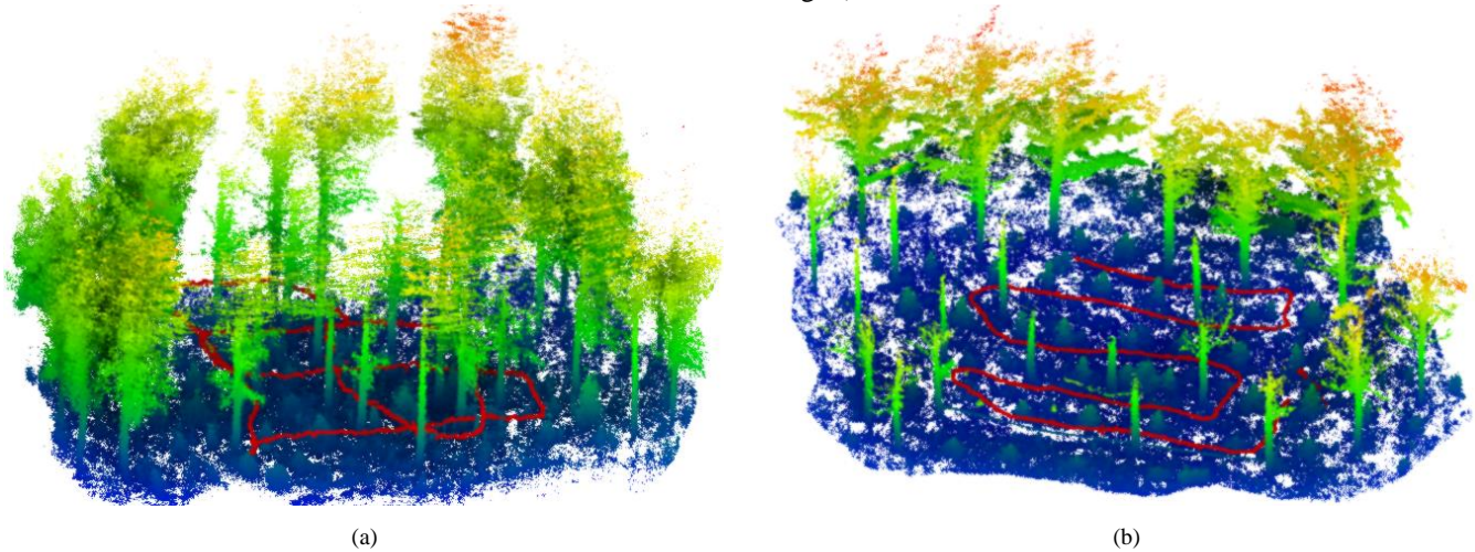
Fig. 6. Forest mapping results. (a) and (b) represent the mapping results of datasets 1 and 2, respectively, where red points represent the trajectories of the BLS system in the test plots.
