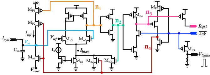
Fig. 1: Neuron circuit.
