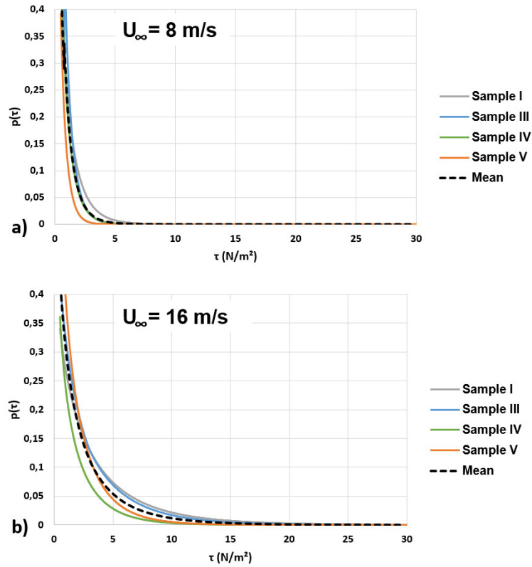
Figure 9. PDF of \tau for the position x = 0.27 m and for a) U_\infty = 8 m/s and b) U_\infty = 16 m/s. The dotted lines represent the average curves that have been chosen to be implemented in the dust emission model.
