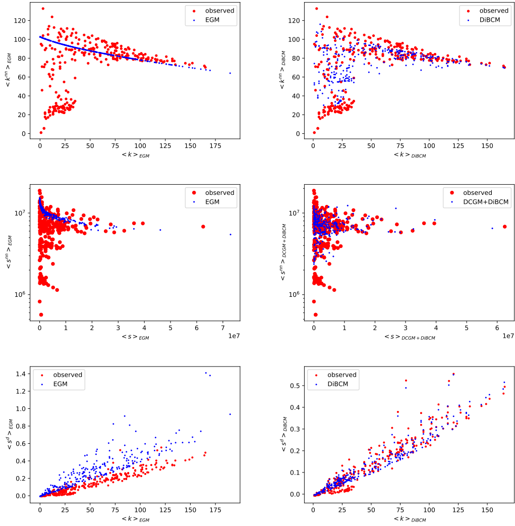
FIG. 5. Maximum entropy models. (left) EGM model; (right) DCGM+DiBCM model; (top) k_i^m = f(k_i) ; (middle) s_i^m = f(k_i) ; (bottom) s_i^d = f(k_i)
