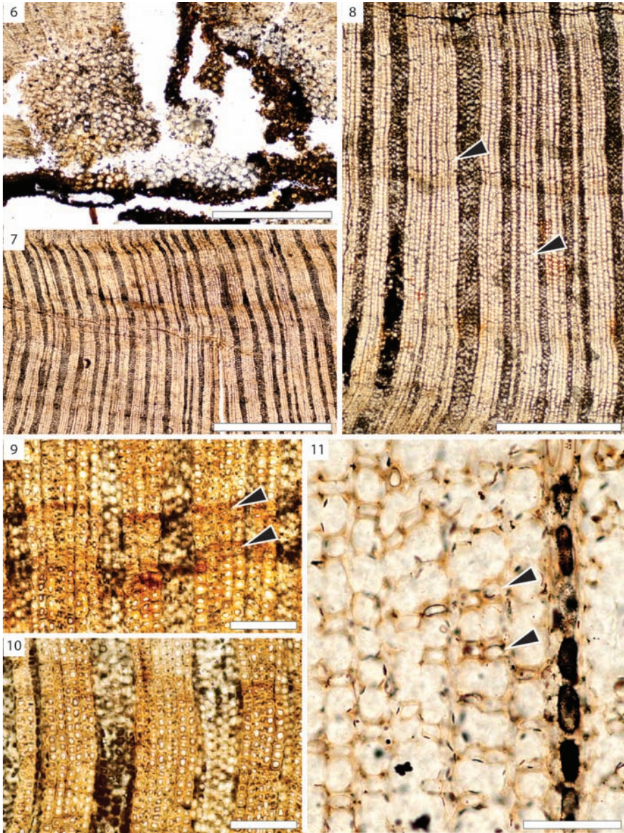
Figure 6–11. Transverse sections of Sherwinoxylon winteroides Boura & Saulnier, sp. nov. – 6: Parenchymatous pith, UP/SCF.17.007. – 7, 8: Homoxylous wood with broad rays, axial parenchyma diffuse-in-aggregates (arrowheads), UP/SCF.17.005. – 9, 10: Thick-walled tracheids; note the indistinct growth rings (arrowheads) marked by 1–3 rows of flattened tracheids with thickened walls, UP/SCF.17.004. – 11: Axial parenchyma diffuse-in-aggregates (arrowheads), UP/SCF.17.003. – Scale bar 6 = 1 mm, 7 = 2 mm, 8 = 500 \mu\text{m} , 9 & 10 = 250 \mu\text{m} , 11 = 100 \mu\text{m} .
