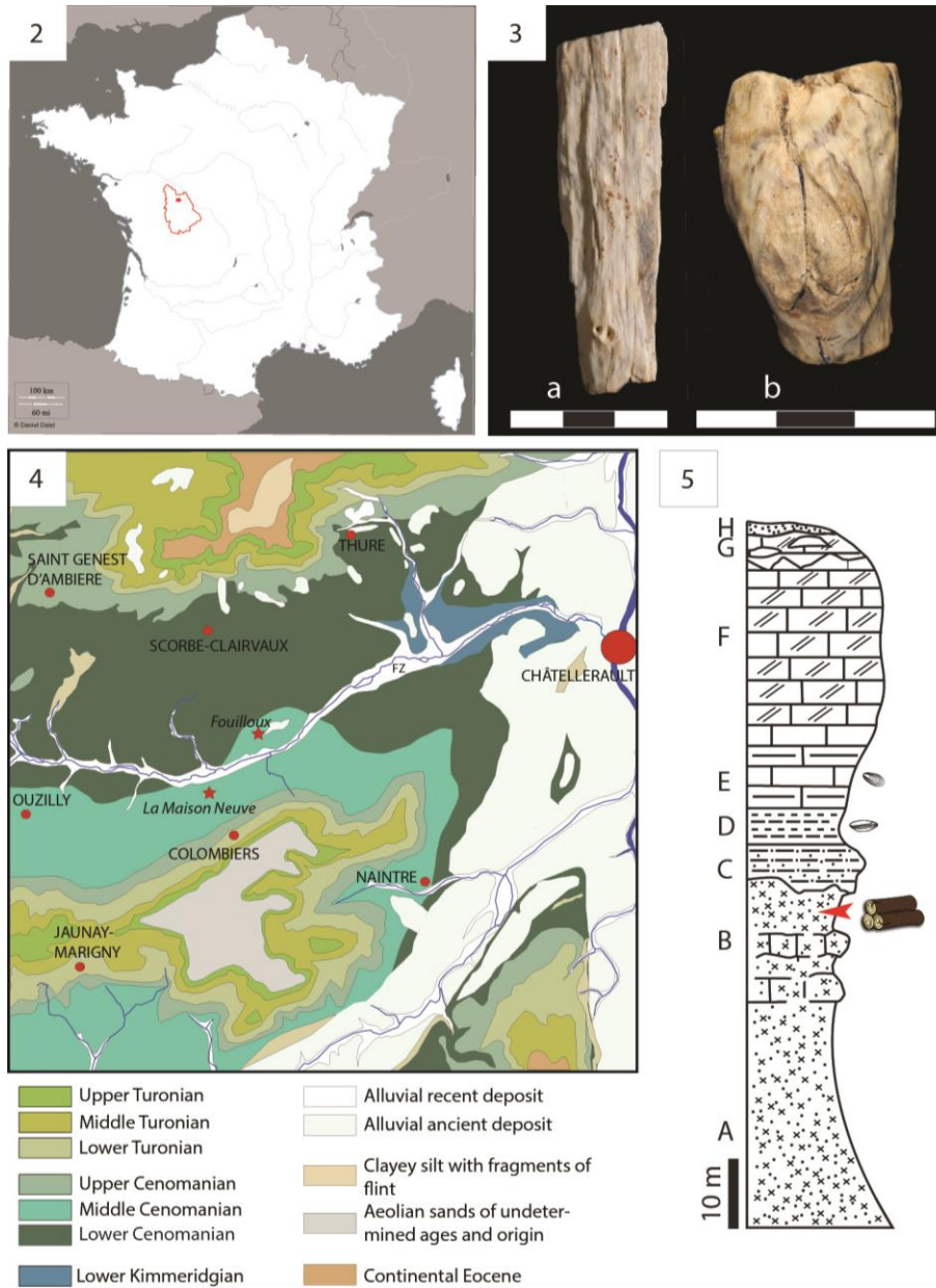
Figs. 2–5. –2 Map of France showing the Vienne department (outline in red), the type locality, Scorbe-clairvaux, is included in the red rectangle. The area represented by this rectangle is magnified in 4; – 3: Two fossil wood samples a = UP.SCF.17.004 and b = UP.SCF.17.007. Scale bars 3 cm. Multiseriate rays are visible to the naked eye. 4- Simplified geologic map showing the two new localities: Fouilloux (Type locality, Scorbe Clairvaux) and 'La Maison Neuve' (Colombiers) are illustrated by red stars. Jaunay-Marigny represents the historical locality where in 1870 the French geologist A. Le Touzé de Longuemar has reported for the first time silicified wood. Modified from Médioni et al. (1974) and Bourguéil et al. (1976); –5: stratigraphic column modified after Gabilly & Cariou (1997): A, claystones and white sandstones of Vierzon (lower Cenomanian); B, green sandstones and C, sandy-claystones of La Pallu (middle Cenomanian); D, plastic claystones and white marlstones with oysters (upper Cenomanian); E, clayey limestones and chalkstones with Inoceramus labiatus (lower Turonian); F, white tufa (micaceous glauconitic chalk, middle Turonian); G–H, altered yellow tufa and clayey sandstones with silicified nodules with plants (Gomez et al. 2018) (upper Turonian). Studied wood remains were collected from the green sandstones and claystones of La Pallu (indicated in B).
