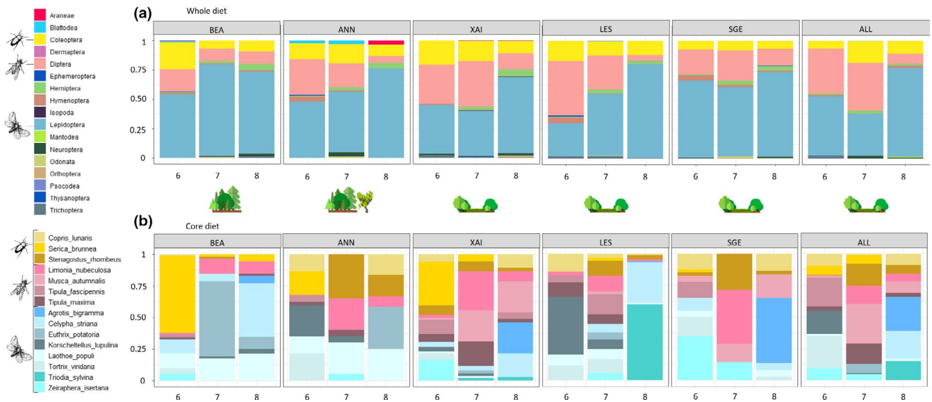
FIGURE 4 Frequency of occurrences in each of the six colonies—sorted according to their coordinates on the Axis.1 of the PCA (Allonne “ALL,” Annepont “ANN,” Beaumont “BEA,” Lessac “LES,” Sainte-Gemme “SGE,” Xaintray “XAI”)—for the three dates of sampling (“6” = June, “7” = July, and “8” = August). (a) The whole diet considered at the order level of taxonomic resolution. (b) The core diet considered at the species level of taxonomic resolution. In both figures, the three most occurrent orders (Lepidoptera, Diptera, Coleoptera) are represented by an icon. The dominant landscapes—as determined by the axes 1 and 2 of the PCA—are indicated for each colony
