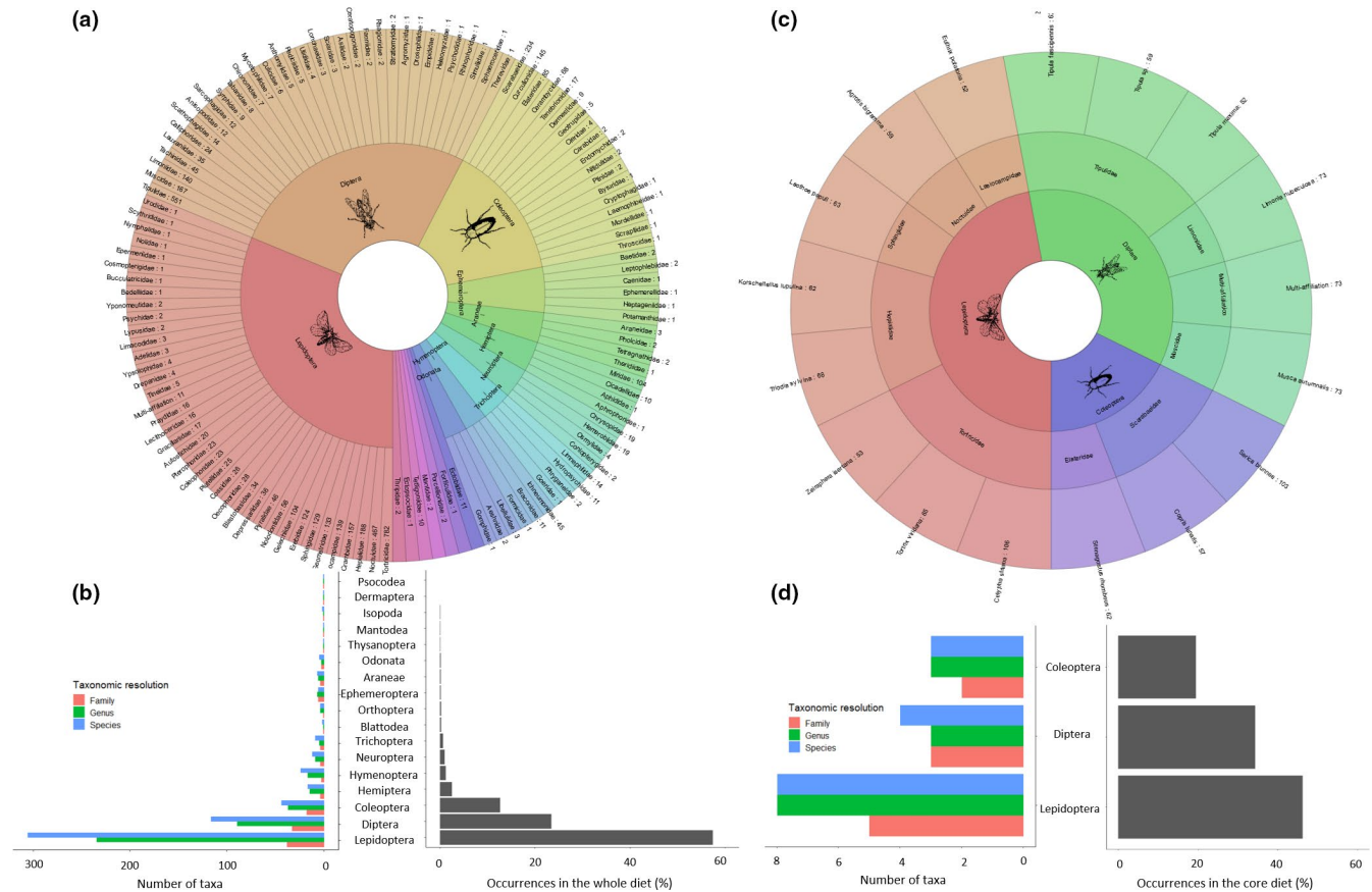
FIGURE 3 Representation of the prey taxonomic diversity detected from R. ferrumequinum guano, considering six colonies and three sampling dates. (a) The two circles represent taxonomic ranks from the families outwards to the order in the center. Numbers correspond to the number of occurrences of each taxonomic family in the whole diet. (b) Taxonomic diversity of the arthropod orders expressed as the number of prey families, genus, species (left), and percentage of occurrences (right) in the whole diet. (c) The circles represent taxonomic ranks from the species outwards to the order in the center considering only the prey with an occurrence frequency > 5%. Numbers correspond to the number of occurrences of each taxonomic family in the core diet. (d) Relative representation of the frequent prey (core diet) expressed as the number of prey families, genus, species (left), and percentage of occurrences (right)
