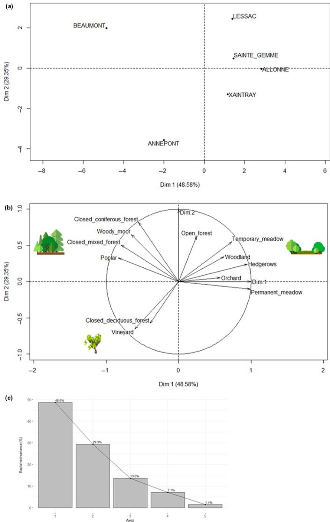
FIGURE 2 Principal Component Analysis (PCA) of twelve features describing the landscape surrounding the colonies (radius = 7 km, surface in hectare). Representation of (a) the six colonies, (b) the landscape variables, and (c) the eigenvalue graph which indicates the percentage of variance explained by each axis of the PCA
