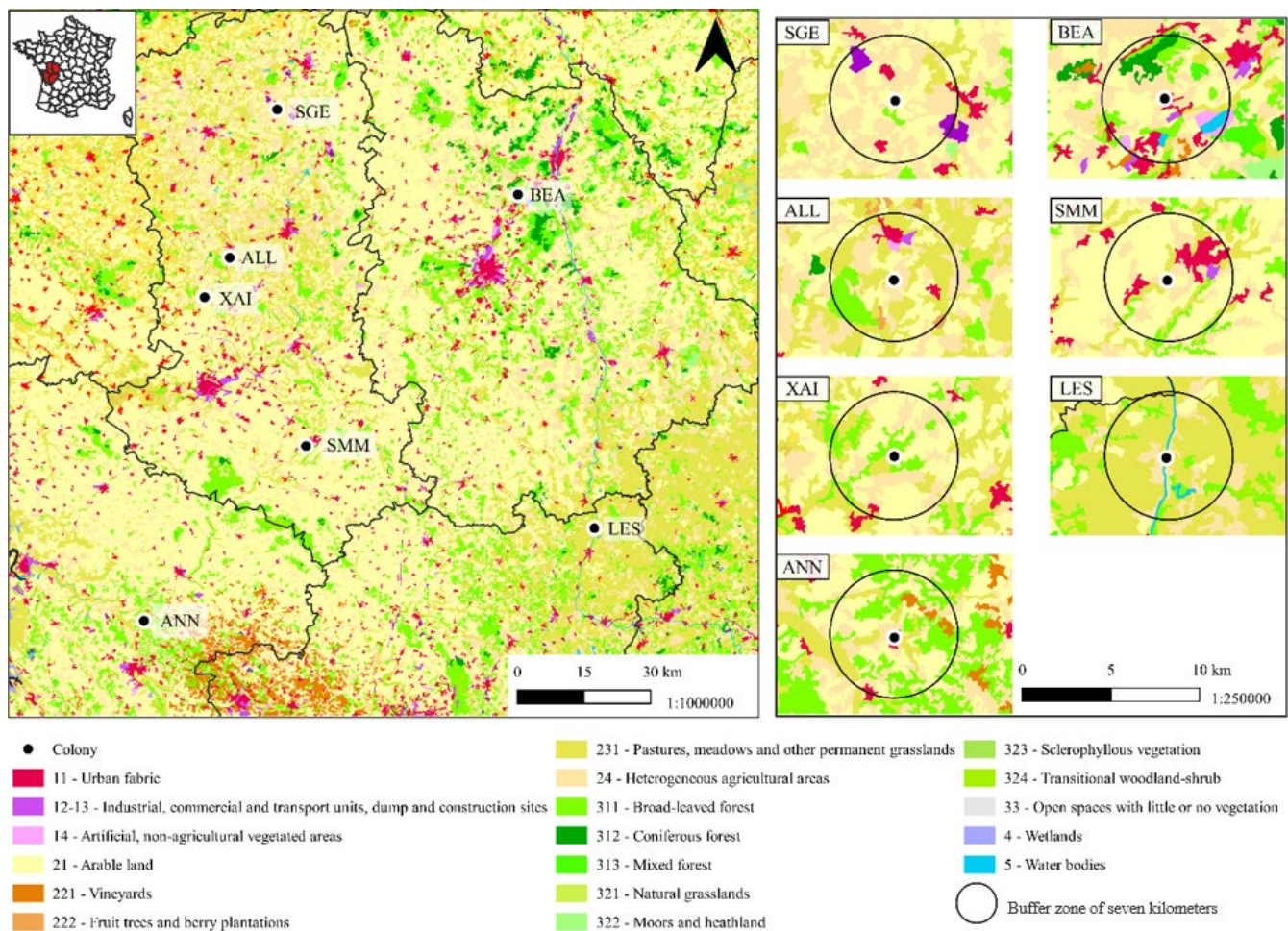
FIGURE 1 CORINE land cover map of the colonies included in this study: Allonne (ALL), Annepont (ANN), Beaumont (BEA), Lessac (LES), Sainte-Gemme (SGE), Saint-Martin-les-Melle (SMM), and Xaintray (XAI). Buffer zone of seven kilometers corresponds to the maximum hunting distance of R. ferrumequinum females during the lactation period
