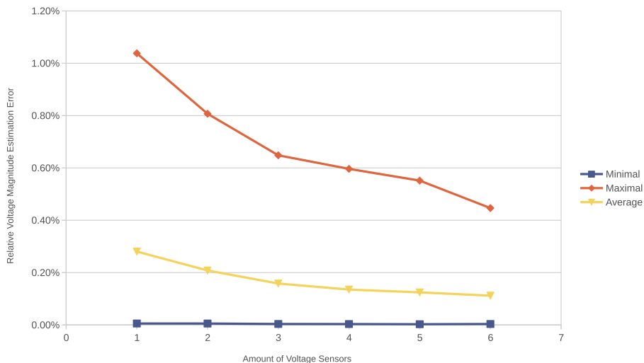
Fig. 4. Performance evaluation on a 111-bus distribution system
