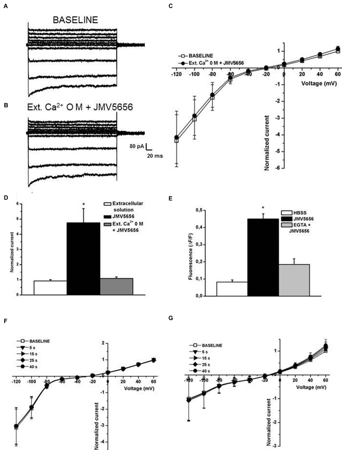
FIGURE 6 | Extracellular and intracellular Ca^{2+} dependence of JMV5656 effect on K_{Ca3.1} channels. (A,B) Representative families of currents traces recorded in N9 cells perfused with the regular extracellular solution (A) and after 40 s of extracellular solution containing 0 mM Ca^{2+} and JMV5656 (B) in a condition of intracellular free calcium concentration of 100 nM. (C) Current/voltage relationship during perfusion with the extracellular solution (baseline, empty symbols) and perfusion containing JMV5656 (filled symbols) but lacking of Ca^{2+} . (D) Normalized current amplitude recorded at +60 mV after 40 s of perfusion with extracellular solution ( n = 11 ), JMV5656 ( n = 9 ), JMV5656 without extracellular Ca^{2+} ( n = 15 ). (E) Cytosolic calcium mobilization, expressed as variation in fluorescence intensity, obtained in N9 cells stimulated with the vehicle only (HBSS), with JMV5656 and with JMV5656 in presence of 1 mM EGTA to chelate the extracellular calcium. (F) Current/voltage relationship obtained in presence of JMV5656 in the extracellular solution and BAPTA 5 mM in the intracellular one ( n = 5 ). (G) Current/voltage relationship obtained in presence of JMV5656 in the extracellular solution and 3 \mu M free intracellular calcium ( n = 16 ); recording were made at selected time points (5, 15, 25, and 40 s). * p < 0.05 vs control group. All data have been obtained in three independent experiments.
