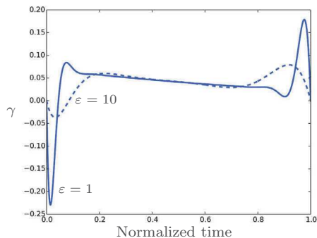
Fig. 3. The air slope \gamma(\cdot) for \varepsilon = 10 (dashed line) and \varepsilon = 1 (solid line).
