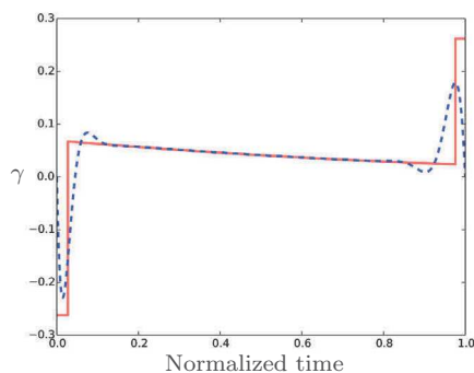
Fig. 5. The air slope \gamma(\cdot) for \varepsilon = 1 (blue dashed line) and \varepsilon = 0 (red solid line). When \varepsilon = 0 , \gamma(\cdot) is the control law of problem (P_0) .
