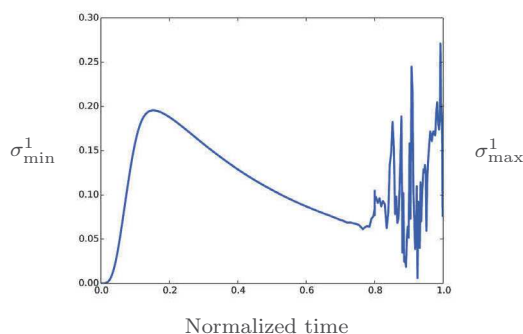
Fig. 7. The singular values \sigma_{\min}^\varepsilon(\cdot) and \sigma_{\max}^\varepsilon(\cdot) for \varepsilon = 1 .
