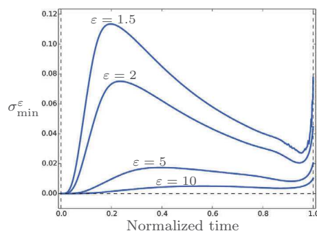
Fig. 6. The singular value \sigma_{\min}^\varepsilon(\cdot) for \varepsilon \in \{1.5, 2, 5, 10\} .
