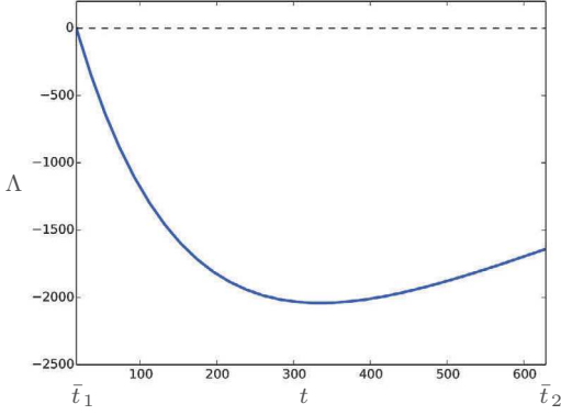
Fig. 2. The determinant \Lambda := \det(J, F_0, F_1) , with J(\bar{t}_1) = F_1(x(\bar{t}_1)) , along the singular arc for the trajectory of the form \sigma_- \sigma_s \sigma_+ associated to \bar{y} .
