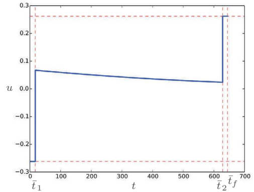
Fig. 1. The control law u(\cdot) = \gamma(\cdot) for the trajectory of the form \sigma_- \sigma_s \sigma_+ associated to \bar{y} .
