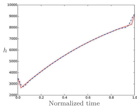
Fig. 4. The altitude h(\cdot) for \varepsilon = 1 (blue dashed line) and \varepsilon = 0 (red solid line).
