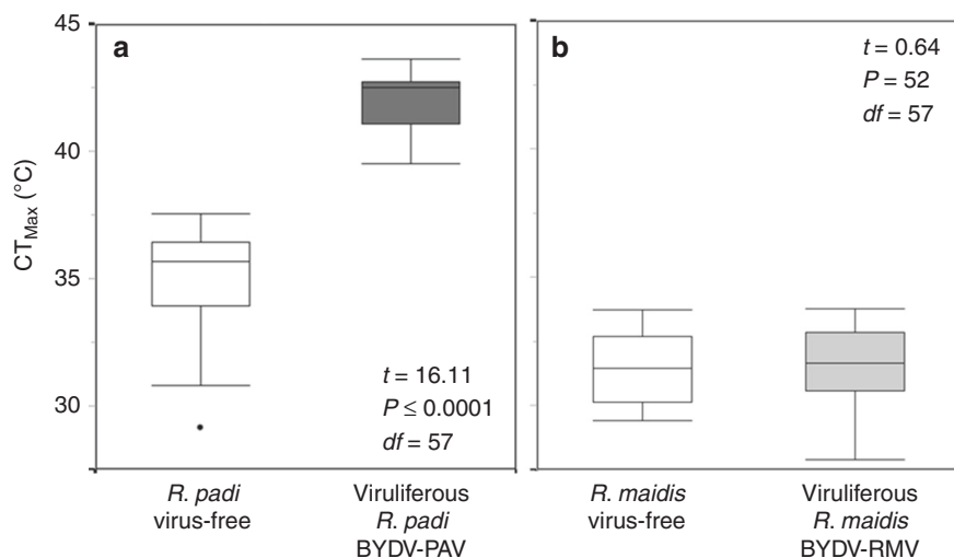
Fig. 3 Upper temperature limit for locomotion ( CT_{Max} ) for viruliferous and virus-free aphid species. CT_{Max} of (a) R. padi and (b) R. maidis . Student's t test (boxplots display median line, interquartile range (IQR) boxes, 1.5 \times IQR whiskers; n = 30 aphids per treatment). Source data are provided as a Source data file.
