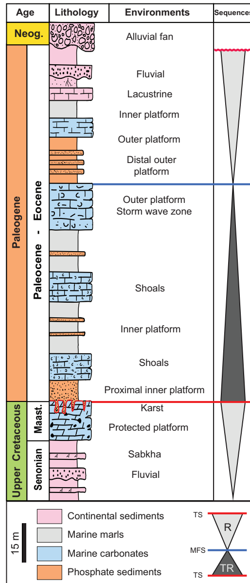
Fig. 2. Synthetic log of the Moroccan High Atlas phosphate-bearing series showing the marine dominated character of the studied sedimentary successions. Depositional sequences are from Chellai et al. (1995). TR: Transgressive hemicycle; R: Regressive hemicycle; TS: Transgressive surface; MFS: Maximum flooding surface.
