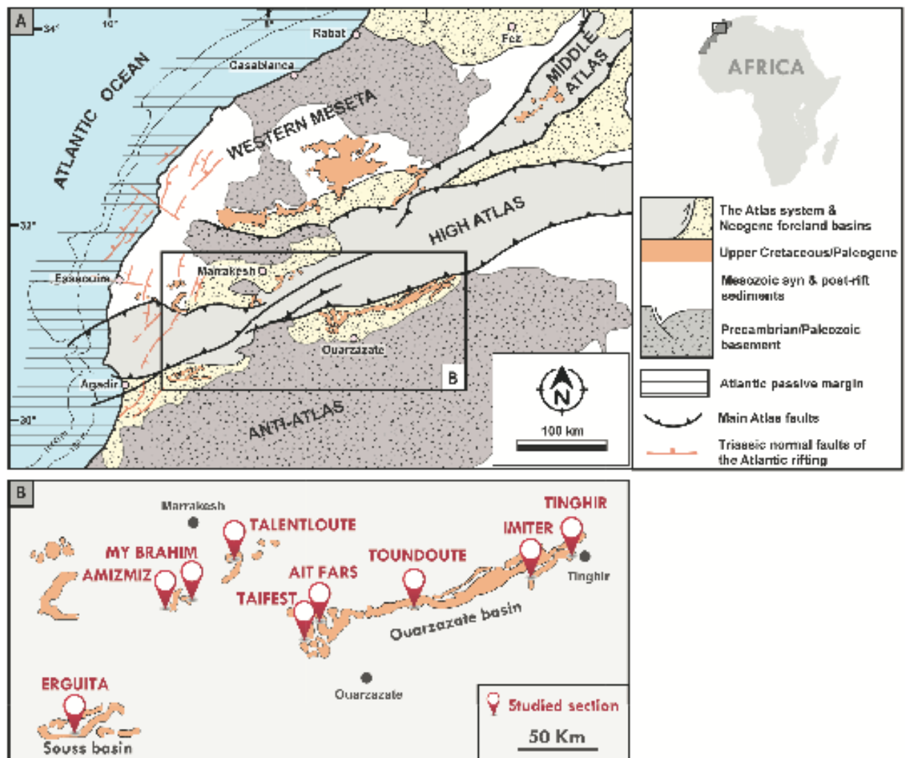
Fig. 1. (A) Simplified structural map of Morocco illustrating the spatial distribution of the Upper Cretaceous-Paleogene phosphate-rich sediments and highlighting the main structural and geodynamic features of the Moroccan Atlas system. Modified after Hafid et al. (2006). (B) Location of the investigated sections along the northern and southern borders of the High Atlas system.
