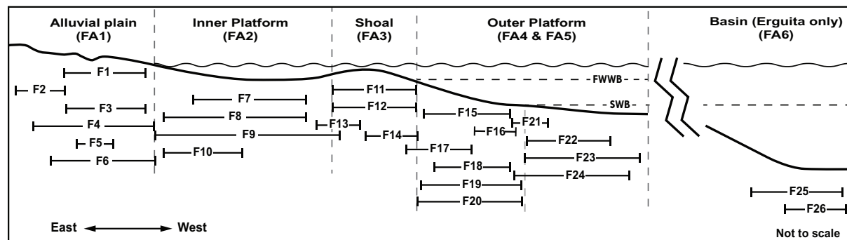
Fig. 6. 2D facies substitution diagram of the studied sedimentary series highlighting the distribution of the defined facies within a shallow-marine platform profile. FWWB: fair-weather wave-base; SWB: storm wave-base.
