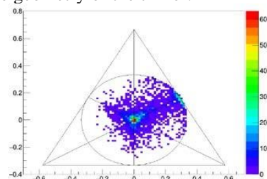
Figure 1. Dalitz plot obtained for the fragmentation of (CO) 3 3+ in three singly charged (CO) + fragments.
