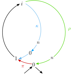
■ Figure 1 First case in proof of Prop. 10
