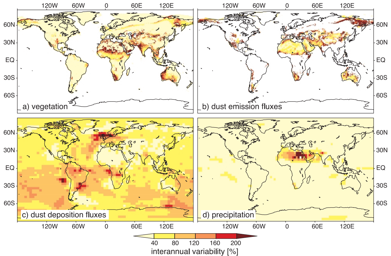
Figure 9. Simulated relative interannual variability (expressed as 1\sigma standard deviation of the 9-year simulation period divided by the long-time mean value) of (a) vegetation cover changes, (b) dust emission fluxes, (c) dust deposition fluxes, and (d) precipitation during the LGM climate.
