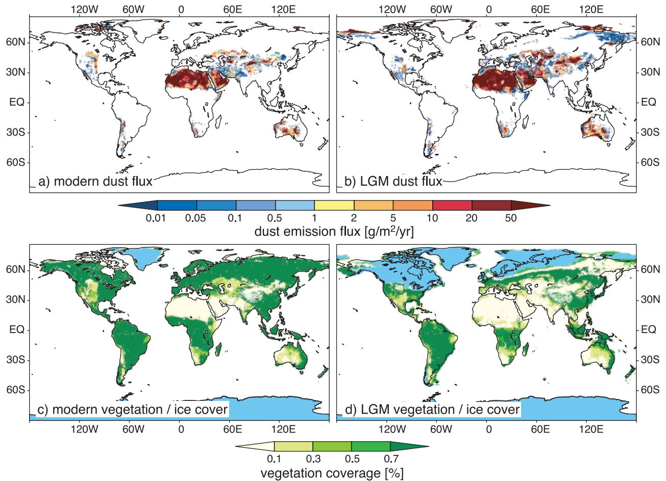
Figure 6. Simulated mean dust emission fluxes for (a) the modern and (b) the LGM climate. Simulated mean ice and vegetation cover fraction for (c) the modern and (d) the LGM climate. Ice coverage is plotted in blue in Figures 6c and 6d.
