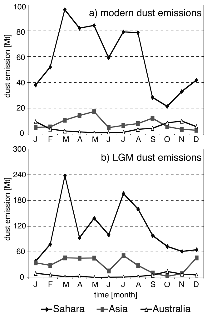
Figure 7. Mean monthly dust emission fluxes (Mt) from the Sahara/Sahel, Asia and Australia for (a) the present and (b) LGM climate. Different scales are used for the magnitude of emissions in Figures 7a and 7b.
