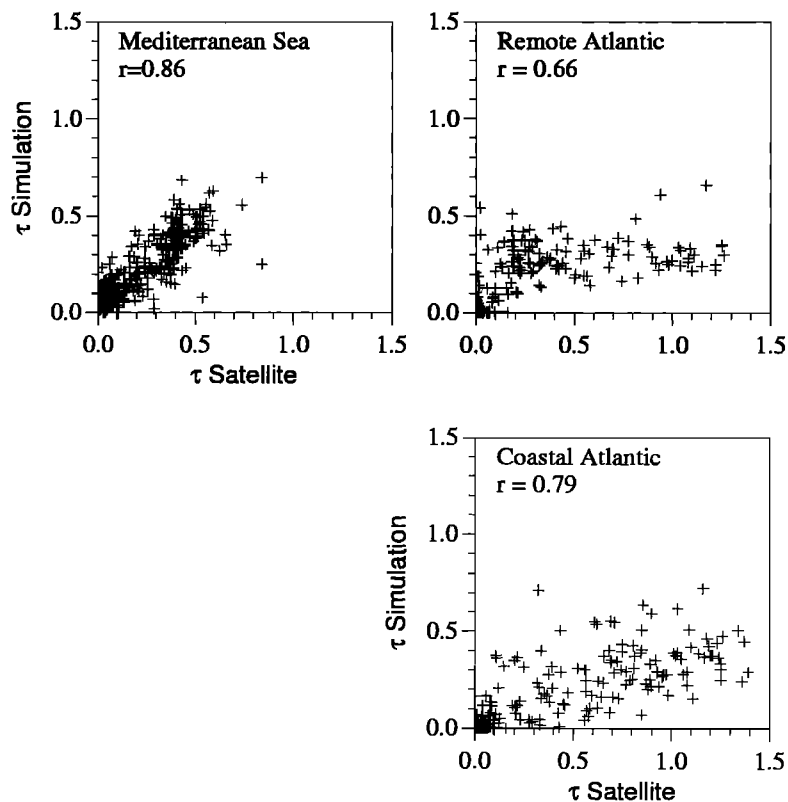
Figure 2: Point-by-point comparison of observed and simulated optical thickness over the whole Mediterranean Sea, and the coastal as well as remote Atlantic as marked in figure 4.
