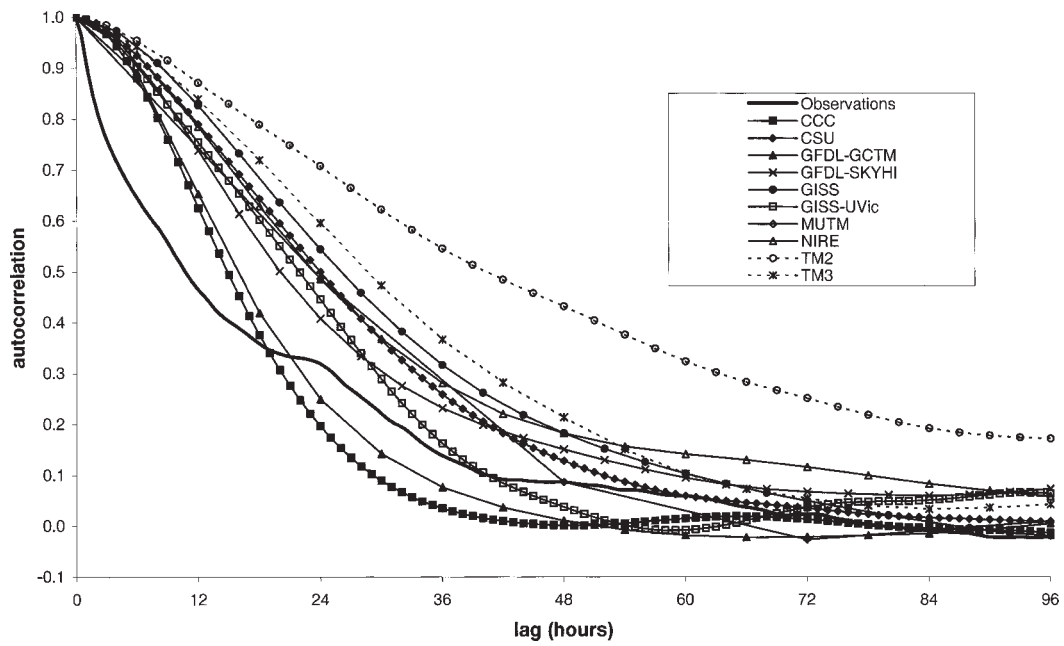
Figure 8b. Autocorrelation function at the WLEF Tower
