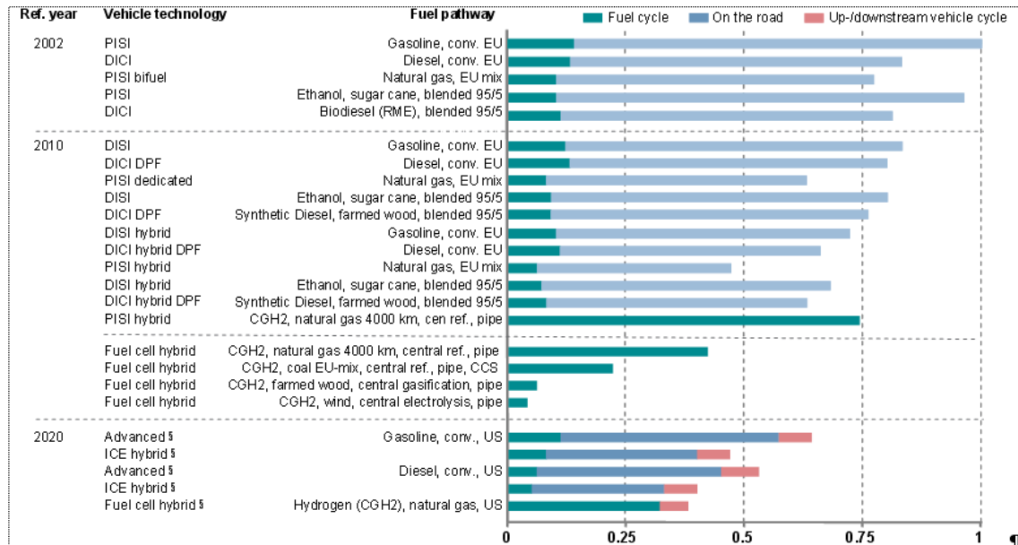
3 Figure 21: Vehicle technologies and alternative fuels: CO 2 -eq emissions well-to-wheels
