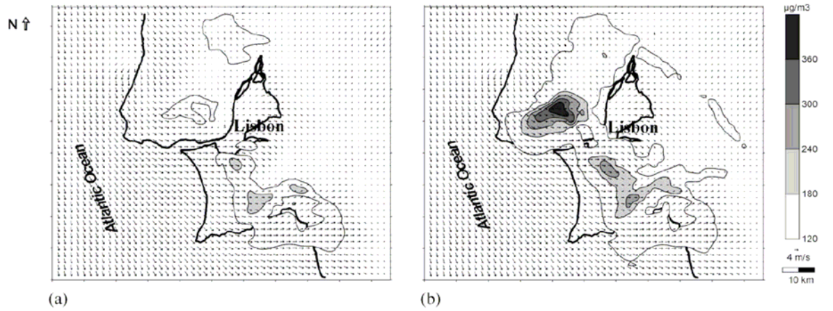
2 3 Figure 9. Simulation results of ozone peak values in July for two emissions scenarios at Lisboa: 4 (A) without traffic emissions; (B) with traffic emissions. (Borrego et al., 2000)
