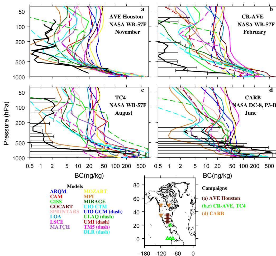
Fig. 9. Model profiles in approximate SP2 BC campaign locations in the tropics and midlatitudes, averaged over the points in the map (bottom). Observations (black curves) are average for the respective campaigns, with standard deviations where available. The Houston campaign has two profiles measured two different days. Mean (solid) and median (dashed) observed profiles are provided for (d). The markers in the map inset denote the location of model profiles in these comparisons with the aircraft measurements that are detailed in Table 7.
