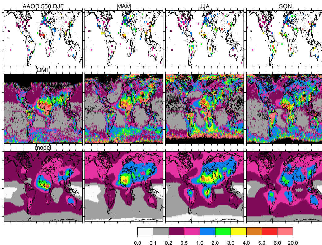
Fig. 6. Seasonal average AAOD ( \times 100 ) for AERONET 550 nm (top), OMI 500 nm (middle), standard GISS model 550 nm (bottom).
