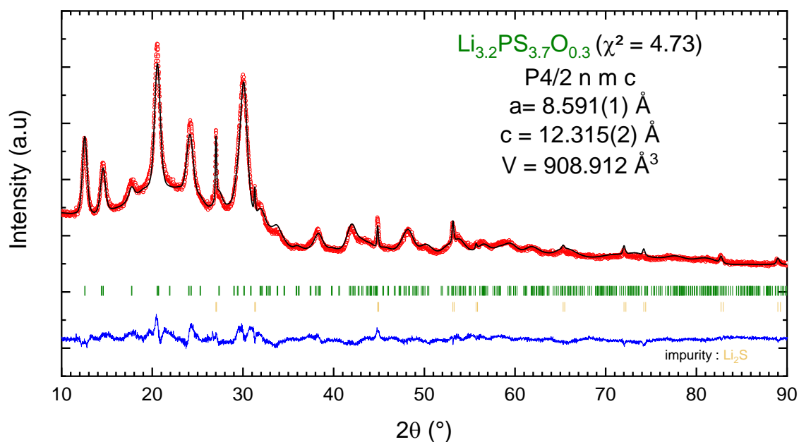
Figure 2. Rietveld refinements of XRD pattern of \text{Li}_{3.2}\text{PS}_{3.7}\text{O}_{0.3} .
