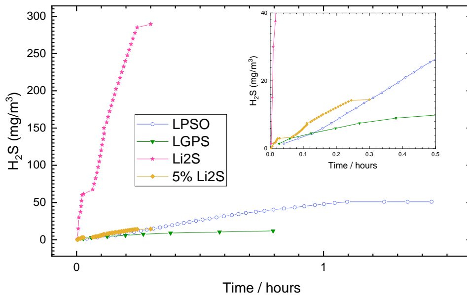
Figure 7. \text{H}_2\text{S} amount generated from \text{Li}_{3.2}\text{PS}_{3.7}\text{O}_{0.3} , \text{Li}_2\text{S} and \text{Li}_{10}\text{GeP}_2\text{S}_{12} compound after exposition to air.
