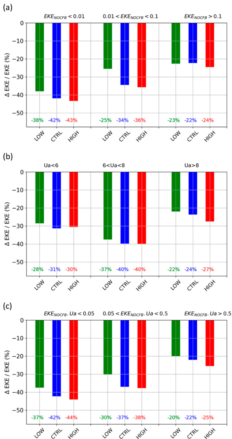
FIG. 3. Percentage of EKE decrease due to current feedback averaged over regions characterized by (a) their EKE level ( m^2 s^{-2} ) in NOCFB simulations (delimited by the black contours in Fig. 1a), (b) their wind speed U_a ( m s^{-1} ), and (c) a combination of wind speed and EKE ( m^3 s^{-3} ).
