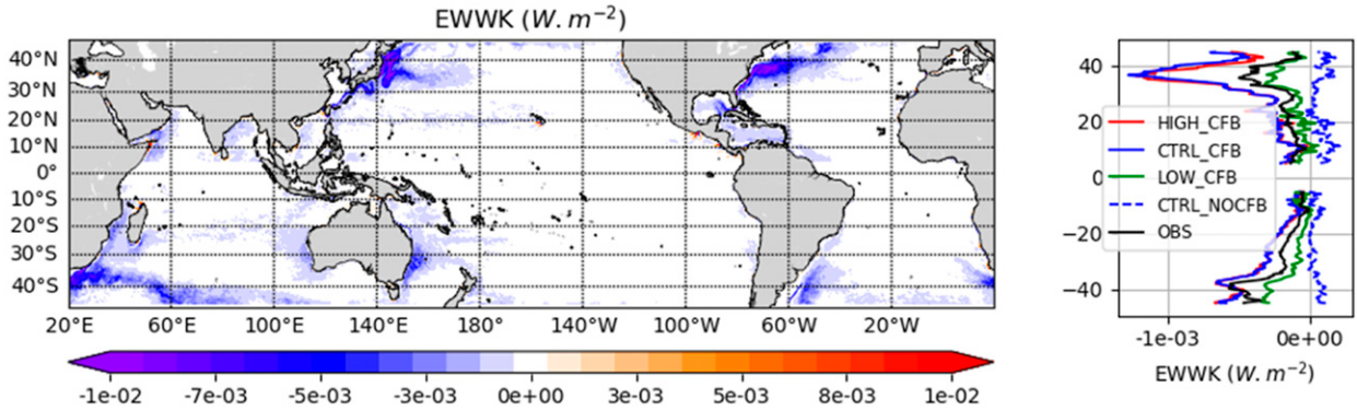
FIG. 4. The 5-yr average of eddy wind work (EWWK; \text{W m}^{-2} ) in the CTRL_CFB simulation. The side plot represents the EWWK zonal average for HIGH_CFB (red), CTRL_CFB (blue), LOW_CFB (green), and CTRL_NOCFB (dashed blue) simulations, and observations (black).
