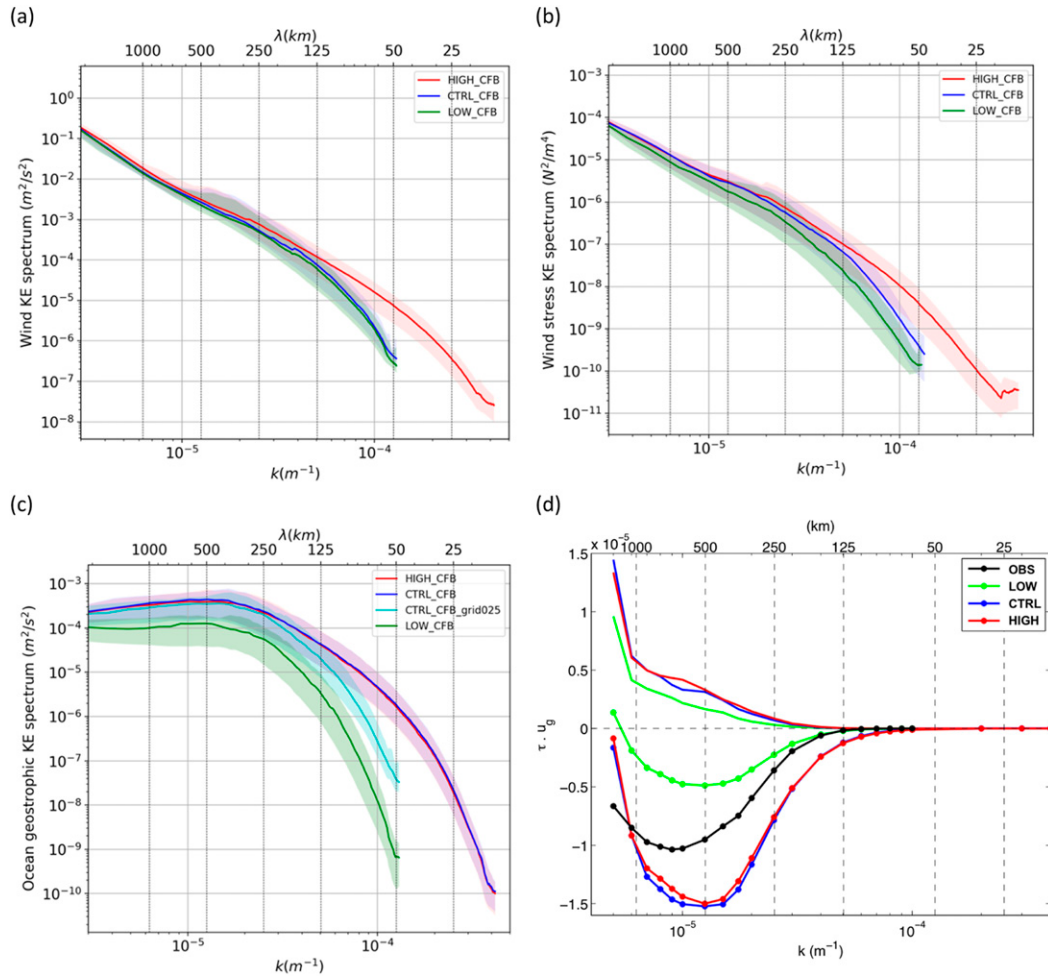
FIG. 7. (a) Wind speed power spectrum, (b) wind stress power spectrum, (c) geostrophic current power spectrum, and (d) cospectrum of the geostrophic wind work ( WWK\rho_0 ) as a function of wavenumber. All spectra are averaged over the whole oceanic domain, and over the 5 years of simulation, for the HIGH (red), CTRL (blue), and LOW (green) simulations. In (a)–(c) CFB simulations are represented. In (d) both CFB (star solid lines), and NOCFB (solid lines) are represented, as well as the observations (black). Note that in the spectral space, wavelengths are considered, and thus the minimal representable wavelength corresponds to two grid points.
