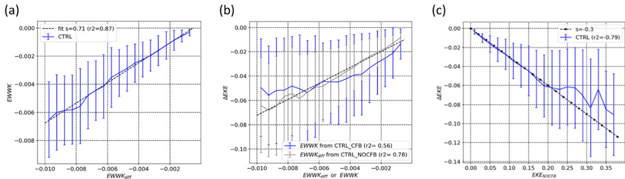
FIG. 5. (a) Regression between analytical eddy wind work difference due to the current feedback ( \text{EWWK}_{\text{diff}} ) computed from CTRL_NOCFB and the actual eddy wind work in CTRL_CFB (EWWK); (b) regression between EWWK (blue) or \text{EWWK}_{\text{diff}} (gray), and the difference of EKE due to current feedback in CTRL ( \Delta\text{EKE} = \text{EKE}_{\text{CTRL\_CFB}} - \text{EKE}_{\text{CTRL\_NOCFB}} ); and (c) regression between EKE in CTRL_NOCFB and \Delta\text{EKE} in CTRL. Dashed lines in (a) and (b) are the linear fits for CTRL_CFB. The star-dashed line in (c) is the linear regression with a slope equal to -0.3 .
