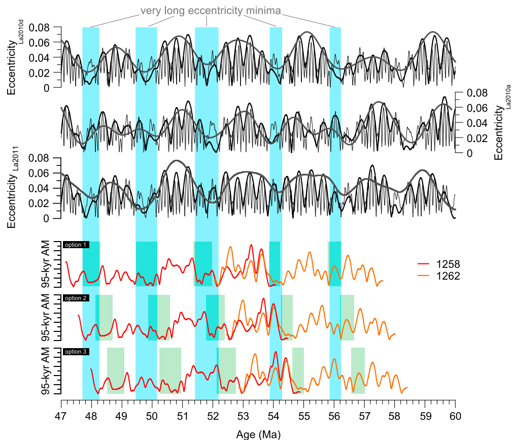
Figure 5. Comparison of the amplitude modulation (AM) of the short eccentricity cycle (95-kyr band) between the La2010d, La2010a, La2011 orbital solutions and Fe intensity data from ODP Sites 1258 (red) and 1262 (orange). For the orbital solutions we also plotted the 405-kyr AM. The 95-kyr AM of Site 1258 and 1262 Fe intensity data are plotted on the three minimal tuning age scale options (Table 3). \sim 2.4 myr minima are highlighted by light blue bars in the orbital solutions and light green bars in the 95-kyr AM of the 1258 and 1262 Fe intensity data. Best match (Table 1) between orbital solution and geological data are obtained using tuning option 1 in the stable interval from 47 to 54 Ma.
