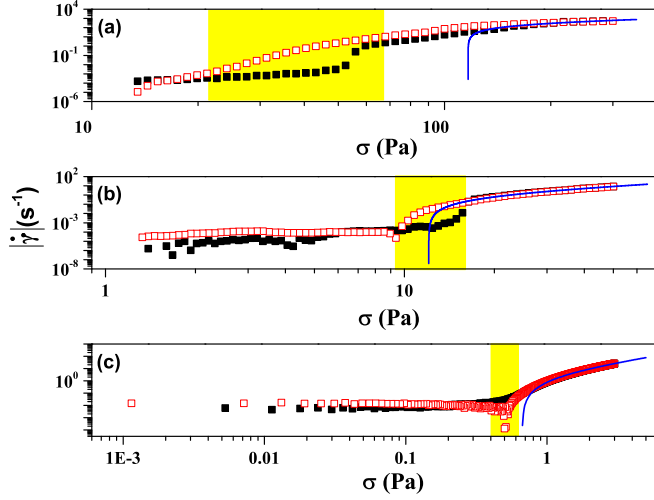
Figure 4. Rheological flow curves measured via controlled stress ramps for various materials: (a) mayonnaise (Carrefour, France) (b) mustard (Carrefour, France) (c) 0.08% (wt) aqueous solution of Carbopol ® 980. For each stress value the response of the material was averaged during t_0 = 10s . The range of applied stresses corresponding to the yielding transition is highlighted in each subplot. The full lines are non linear fitting functions according to the Herschel-Bulkley model. The full/empty symbols in each panels refer to the increasing/decreasing branches of the stress ramp schematically illustrated in Fig. 3(a).
