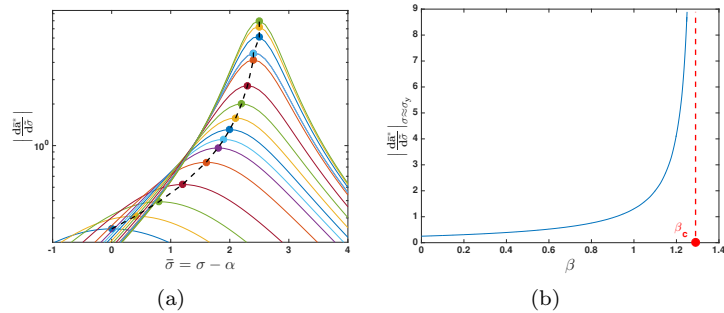
Figure 19. (a) Dependence of the slope of the dependence of \bar{a}^* on the applied stress on the yield stress for various values of \beta ranging from 0 to 2 ( \beta increases from bottom to top). (b) Dependence of the maximum value of the slope \left. \frac{d\bar{a}^*}{d\tilde{\sigma}} \right|_{\tilde{\sigma} \approx \sigma_y} given by Eqn. 24 calculated around the yield point on the interaction parameter \beta .
