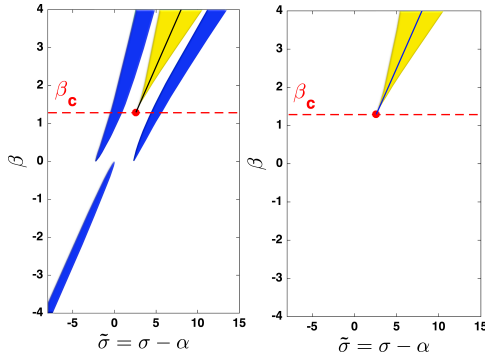
Figure 14. Four real roots of the quartic occur in the shaded regions (blue and yellow) over \tilde{\sigma} = \sigma - \alpha and \beta is shown in the left panel. The black line is \beta = \tilde{\sigma}/2 started at (2.589145, 1.2945725) . The parameter space with only three distinct real roots in [0, 1] is shown in the right panel.
