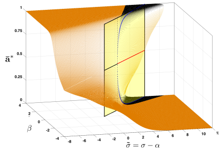
Figure 15. The fixed points \bar{\mathbf{a}}^* as a set-valued function of the parameters \tilde{\sigma} = \sigma - \alpha and \beta . The blue, black and azure points are the stable fixed points while the red and green points are the unstable fixed points of the system. There is a pitch-fork bifurcation along \tilde{\sigma} = 2\beta that starts at (2.589145, 1.2945725) where the fixed point at 0.5 becomes unstable with two stable fixed points on either side.
