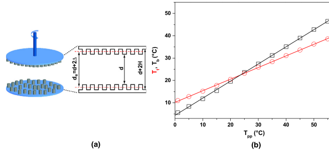
Figure 36. (a) Schematic illustration of the cleated parallel plate geometry. (b) Temperature calibration measurements. The symbols are: circles - the top plate, squares - the bottom plate. A thermorheologically simple silicon oil with a known activation energy has been used.
