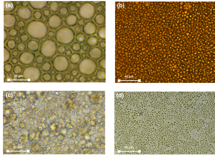
Figure 6. Micrographs of several yield stress materials: (a) commercial shaving gel (Gillette Series) (b) mayonnaise (Carrefour, France) (c) 5% bentonite in water (d) suspension of Chlorella Vulgaris unicellular micro alga (reproduced from Ref. Souliès et al. (2013))
