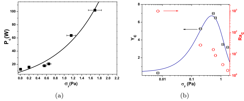
Figure 46. (a) Dependence of the critical heating power P_c corresponding to the onset of the Rayleigh-Bénard convection on the yield stress \sigma_y of the Carbopol ® solution. The line is an exponential fit. (b) Dependence of the critical yield number Y_c (squares, bottom-left axis) and of the critical Rayleigh number Ra_c (circles, bottom-right axes) on the yield stress \sigma_y .
