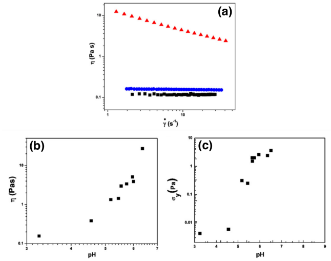
Figure 31. (a) Strain rate dependence of the effective viscosity of the two reacting fluids: circle - displaced Carbopol solution at pH = 3 , squares - displacing sucrose solution at pH = 13 , triangles - neutralised Carbopol ® solution ( pH = 7 ). (b) pH dependence of the viscosity of the Carbopol ® solution measured at \dot{\gamma} = 1 \text{ s}^{-1} . (c) pH dependence of the yield stress of the Carbopol ® solution.
