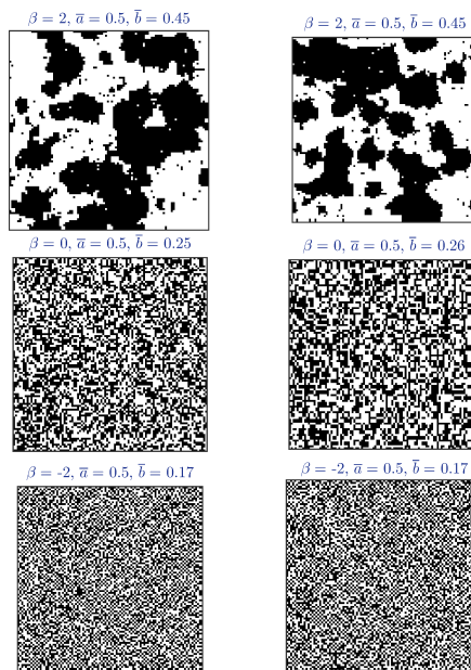
Figure 11. Effect of \beta on preferred energy minimising configurations. Two sample configurations are shown for each \beta \in \{-2, 0, +2\} over a toroidal square lattice of 100 \times 100 sites. Sites in phase 0 and 1 are shown in black and white, respectively, at the solid-fluid interface when \bar{a} \approx 1/2 .
