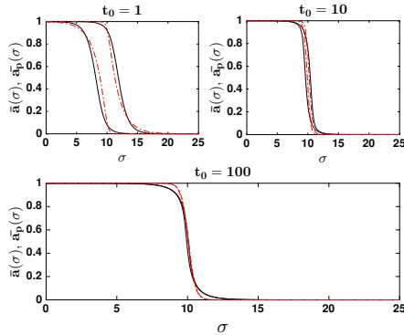
Figure 17. Comparison between ODE approximation and the PMM by Putz and Burghilea Putz and Burghilea (2009) detailed in Sec. 2 for different holding times t_0 . ODE model with \alpha = 8 and \beta = 1 , PMM with k_d = k_r = 0.3 , w = 0.5 and \sigma_y = 10 . Full lines are the ODE approximation and broken lines the PMM.
