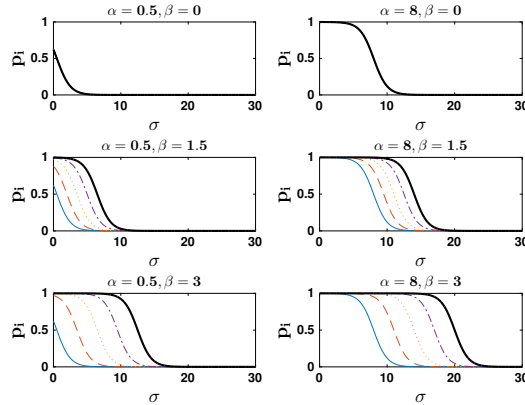
Figure 9. Plots of p_i , the probability that site s with i = x_{N_s} neighbors in phase 1, is also in phase 1, as a function of external stress \sigma for different values of \alpha , \beta . From the plots it is clear that \alpha is a location parameter while \beta controls the scale of the relative difference between p_i 's.
