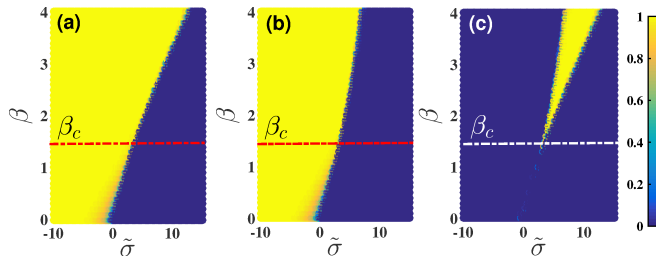
Figure 10. The value of \bar{a} at rescaled time t = 100 from Monte Carlo simulations of the Gibbs field for fixed parameters (\tilde{\sigma}, \beta) when initialized from \mathbf{1} (panel (a) ) and from \mathbf{0} (panel (b) ). The difference in \bar{a} between the sub-plots (a) and (b) is shown in panel (c) . The horizontal dashed lines indicate the critical value of the interacting parameter \beta_c (see the discussion in the text).
