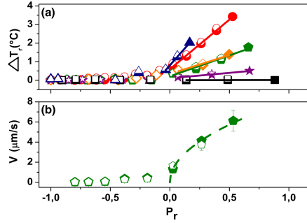
Figure 45. (a) Dependence of the reduced temperature \Delta T_r on the reduced power P_r for various Carbopol concentrations, see Fig. 44. The full lines are linear fitting functions. (b) Dependence the DPIV measured amplitude of the convection pattern V on the reduced power P_r . The line is nonlinear fit function according to the Landau theory of imperfect bifurcation, Eq. 48.
