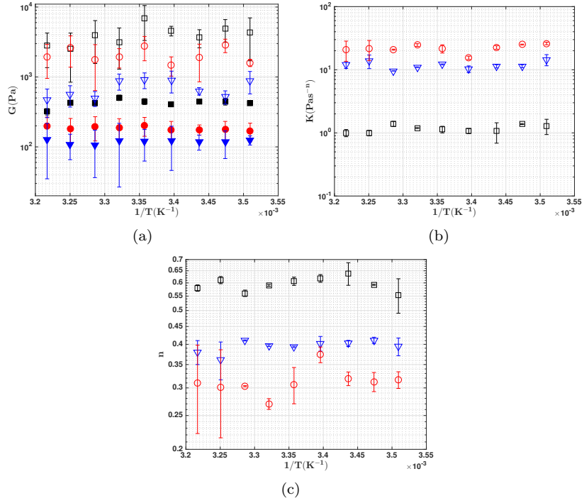
Figure 38. (a) Temperature dependence of the elastic moduli, measured from the increasing (the empty symbols) and decreasing (the full symbols) branches of the controlled stress ramp. (b) Temperature dependence of the consistency. (c) Temperature dependence of the power law index. The symbols in each panels refer to different Carbopol ® weight concentrations: squares - c = 0.1\% , triangles - c = 0.15\% , circles - c = 0.2\% .
