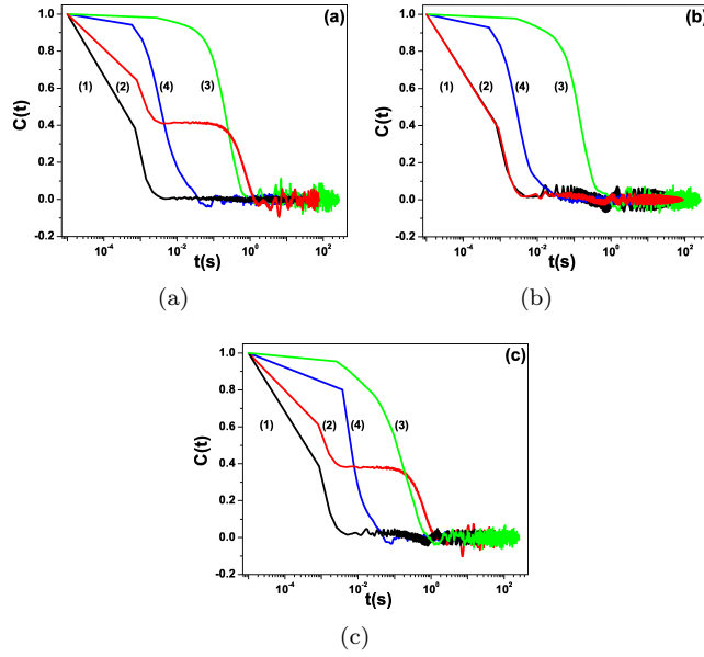
Figure 26. Correlation functions measured for a 0.1% solution Carbopol ® at three different radial positions: (a) r/R=-0.75 (b) r/R=0 (c) r/R=0.75 . The data sets in each panel are: (1) Re_G = 397 , (2) Re_G = 914 , (3) Re_G = 2238 , (4) Re_G = 3309 .
