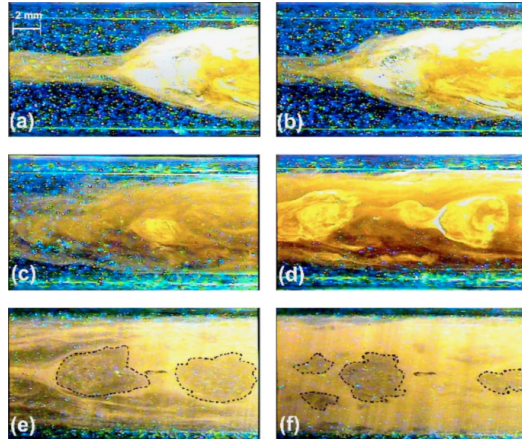
Figure 33. [(a) - (f)]Fluorescent images of the interface in a reactive displacement: displacing fluid - 65% saccharose solution, displaced fluid- 0.1% Carbopol ® in 66% saccharose solution. [(e) - (f)] Fluorescent flow images long after the entrance of the unstable interface in the field of view; the images are separated in time by approximately 5 s. The dotted lines highlight gelled structures tumbling downstream. The direction of the flow in each panel is from right to left.
