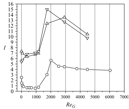
Figure 23. Turbulence intensity measured at r/R = 0 (circles), r/R = -0.75 (up triangles) and r/R = 0.75 (down triangles) for a 0.1% (wt) solution of Carbopol ® 940.
