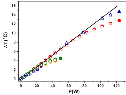
Figure 44. Dependence of temperature gradient on the heat flux for six values of the Carbopol ® concentration: ( \triangle , \blacktriangle ) - c = 0.11\%wt , ( \circ , \bullet ) - c = 0.1\%wt , ( \square , \square ) - c = 0.08\%wt , ( \diamond , \diamond ) - c = 0.075\%wt , ( \star , \star ) - c = 0.06\%wt , ( \square , \blacksquare ) - c = 0.05\%wt . The full/empty symbols refer to increasing/decreasing heat flux. The full line is a linear fit.
