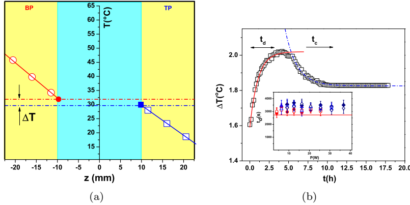
Figure 41. (a) Temperature measurements within the bottom plate BP (the empty circles) and within the top plate TP (the empty squares). The full lines are linear fitting functions and the full symbols are the linear extrapolations of the temperature measurement at the contact points with the fluid. (b) Time series of the temperature difference \Delta T . The full line is a nonlinear fit by Eq. 5. t_d stands for the characteristic thermal diffusion time. The dash-dotted line is a fit according to Eq. 6. t_c stands for the characteristic slowing down time. The dependence of the thermal diffusion time t_d on the heating power P measured for three Carbopol ® solutions with the concentrations c = 0.06\% , 0.075\% , 0.08\% for both increasing (full symbols) and decreasing (empty symbols) heating powers is presented in the inset. The full line is the theoretical estimate, t_d \approx 2730s (see text).
