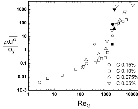
Figure 27. Axial Reynolds stresses normalized by yield stress for four different concentration levels of Carbopol ® . The filled symbols indicate points where the flow becomes transitional, with puffs/slugs first observed.
