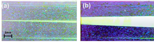
Figure 32. Example fluorescent images of the interface in an experiment from control sequence: displacing fluid 65% saccharose solution, displaced fluid - 66% saccharose solution. The flow rate \hat{Q} = 0.145\text{ml/s} . The two images are separated in time by 5s.
