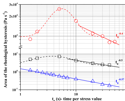
Figure 5. Dependence of the hysteresis area on the characteristic forcing time t_0 (see text for description) measured with several yield stress materials via controlled-stress flow ramps: circle ( \circ ) - mayonnaise (Carrefour, France), square ( \square ) - mustard (Carrefour, France), up triangle ( \triangle ) - 0.08% (wt) aqueous solution of Carbopol ® 980. The dashed lines are log-normal fitting functions (see text for the discussion), the full lines are power law fitting functions indicated in the inserts.
