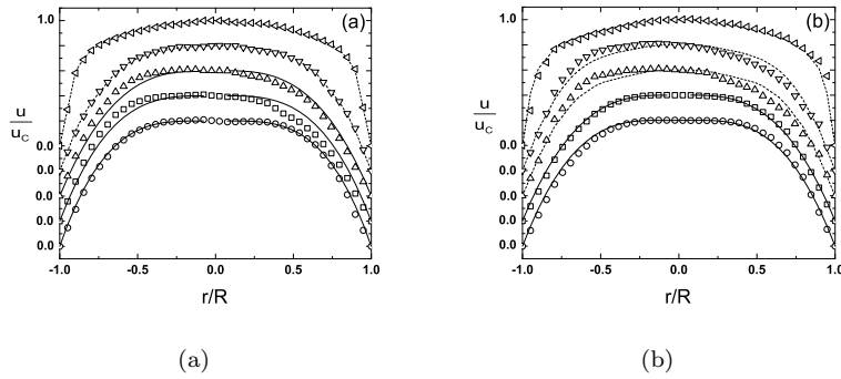
Figure 22. The transversal profiles of the time averaged velocity \bar{u} for 0.1% (wt) Carbopol: (a) Re_G=378(\circ) , 937( \square ), 1160( \triangle ), 1735( \nabla ) and 2920( \triangleleft ) (b) Re_G=397(\circ) , 914( \square ), 2001( \triangle ), 2238( \nabla ) and 2612( \triangleleft ). These data are from replicate tests obtained from similar experimental conditions.
