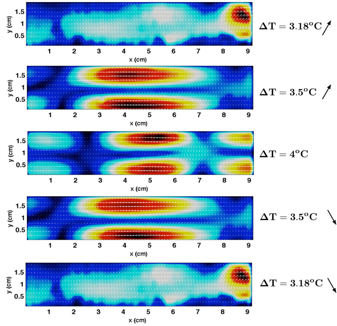
Figure 43. Evolution of the flow patterns corresponding to several values of the integral temperature difference \Delta T indicated in the inserts. The up/down arrows indicate the increasing/decreasing branch of the heating ramp. The false colour map refers to the absolute value of the flow velocity. A 0.08% Carbopol ® solution was used and the onset of the Rayleigh-Bénard convection corresponds to \Delta T_c = 2.58^\circ C .
