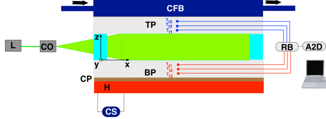
Figure 40. Schematic view of the experimental setup L - solid state laser, CO - cylindrical optics block, CP - copper plate, TP - top plate, BP - bottom plate, CFB - cooling fluid bath, A 2 D - analogical to digital signal conditioning block, RB - reference box.
