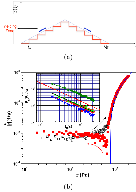
Figure 3. 3(a) Schematic illustration of the controlled stress flow ramp 3(b) Rheological flow curve measured via the controlled stress ramp illustrated in Fig. 3(a) for a 0.1% (wt) solution of Carbopol ® 940. The full line is a non linear fitting functions according to the Herschel-Bulkley model. The full/empty symbols refer to the increasing/decreasing branches of the stress ramp schematically illustrated in Fig. 3(a). The inset presents the dependence of the hysteresis area on the characteristic forcing time t_0 . The full line in the inset is a guide for the eye P_h \propto t_0^{-1} .
