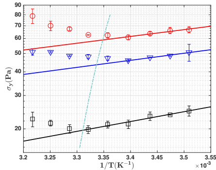
Figure 39. Temperature dependence of the yield stress measured for three distinct values of the Carbopol ® concentration: squares - c = 0.1\% , triangles - c = 0.15\% , circles - c = 0.2\% . The dashed line marks the transition from an Arrhenius temperature dependence to a non-Arrhenius one.
