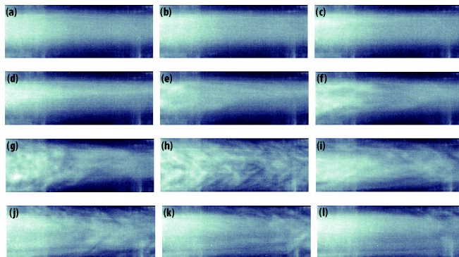
Figure 24. Instant puff images taken for 0.075% solution of Carbopol ® 940 at Re_G = 1850 at different time instants: (a) t = 130ms , (b) t = 225.5ms , (c) t = 255.5ms , (d) t = 320ms , (e) t = 422.5ms , (f) t = 447.5ms , (g) t = 497.5ms , (h) t = 600ms , (i) t = 755ms , (j) t = 1117.5ms , (k) t = 1155ms and (l) t = 1187.5ms .
