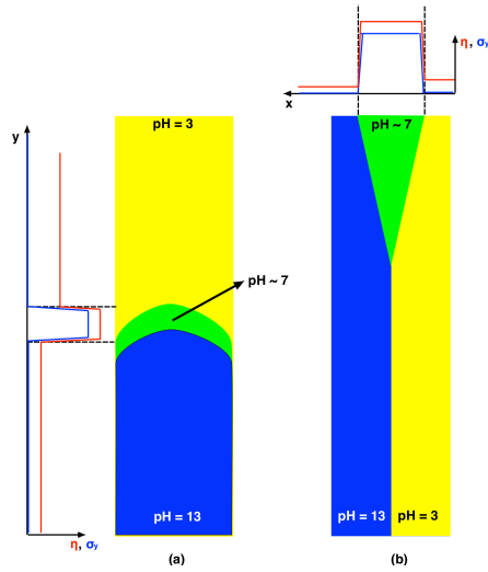
Figure 30. Schematic overview of the reactive flow configurations: (a) displacement configuration (b) Hele-Shaw parallel flow configuration. The colours in each panel refer to the pH of the fluid - see text for description.
