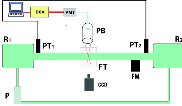
Figure 21. Schematic view of the experimental setup: \mathbf{R}_{1,2} - fluid reservoirs, \mathbf{P} - pump, \mathbf{FM} - flow meter, \mathbf{PT}_{1,2} - pressure transducers, \mathbf{FT} - fish tank, \mathbf{CCD} - digital camera, \mathbf{PB} - laser Doppler velocimetry probe, \mathbf{PMT} - photomultiplier, \mathbf{BSA} - burst spectrum analyzer.
