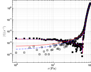
Figure 20. Flow curve measured for increasing (empty symbols) and decreasing (full symbols) values of the applied stress. The full line is a fit by the model by Putz and Burghilea Putz and Burghilea (2009) and the dashed line is the prediction of the nonlinear dynamical system model.
