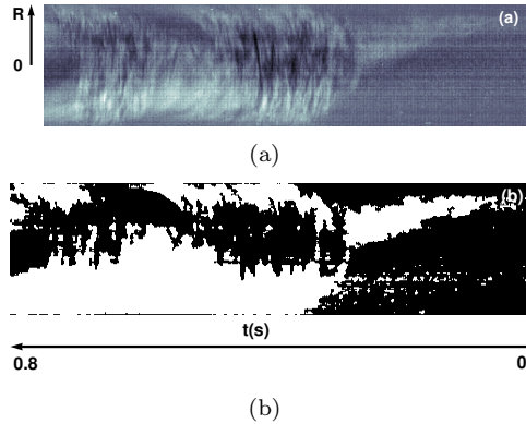
Figure 25. Space time plot measured with a 0.075%(wt) Carbopol ® at Re_G = 1850 (a) obtained from raw images (a) obtained from filtered, background subtracted and binarised images. The puff length is \approx 1.69 m . The images sequence consisted of 320 frames.
