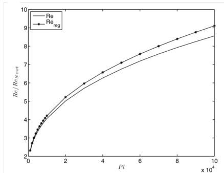
Figure 29. Normalised critical Re for increasing Pl .
