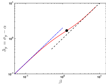
Figure 18. Dependence of the approximate yield stress shifted by the site specific threshold \tilde{\sigma}_y = \sigma_y - \alpha on the interaction parameter \beta . The dashed line is \tilde{\sigma}_y = \beta and the dash-dotted line is \tilde{\sigma}_y = 2\beta . The circles marks the critical point corresponding to \beta_c \approx 1.3 .
