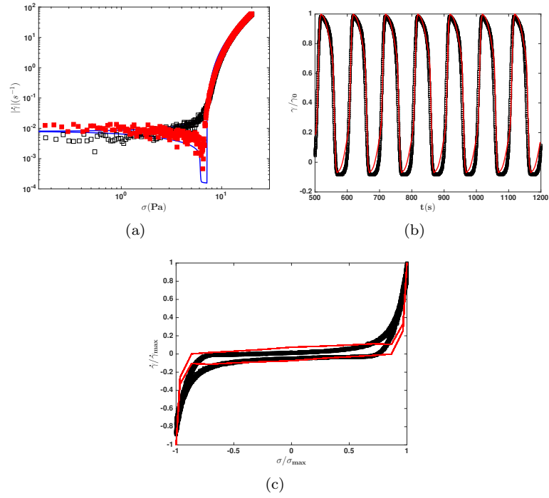
Figure 7. 7(a) Rheological flow curve measured via the controlled stress ramp illustrated in Fig. 3(a) for a 0.1% (wt) solution of Carbopol 940. The full/empty symbols refer to the increasing/decreasing branches of the stress ramp schematically illustrated in Fig. 3(a) 7(b) Normalised strain measured during a controlled stress oscillatory sweep. 7(c) Lissajoux figure corresponding to the controlled stress oscillatory sweep. The full line in each panel is the prediction of the model.
