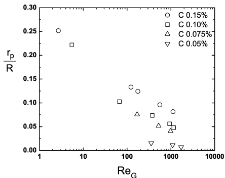
Figure 28. Plug radius normalized by pipe radius for four different concentration levels of Carbopol ® indicated in the insert.
