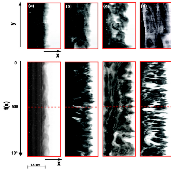
Figure 35. Space - time diagrams measured at a fixed driving pressure drop \Delta p = 500 Pa at several locations downstream: (a) y = 3.2 cm , (b) y = 14 cm , (c) y = 17 cm , and (d) y = 35 cm . The flow patterns have been visualized using the laser induced fluorescence (LIF) technique. LIF flow images acquired in the horizontal plane corresponding to each space - time diagram are presented on the top row. The dotted lines in the bottom row indicate the time instant when the LIF flow images have been acquired. The concentration of Carbopol ® in the acid fluid was 0.1%.
