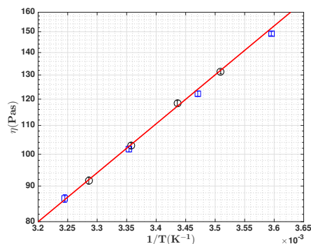
Figure 37. Validation of the cleated geometry and stress correction. The symbols are: circles- cone and plate geometry, squares - the cleated geometry illustrated in Fig. 36(b). A thermorheologically simple silicon oil with a known activation energy has been used.
