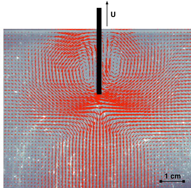
Figure 2. The Landau-Levich flow problem: instantaneous flow field around a rigid plate being withdrawn at constant speed from a bath filled with a Carbopol ® gel.
