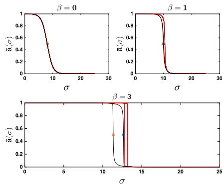
Figure 16. Gibbs field and ODE approximation simulations with \alpha = 8 and \beta \in \{0, 1, 3\} . The stress was increased from 0 to 25 in units of 0.01 and decreased back to 0 with a holding time of t_0 = 1000 (nearly asymptotic state for each distinct stress) as the site configuration varied from \mathbf{1} to \mathbf{0} and then back to \mathbf{1} . The curves with the symbol ( \square ) are the ODE simulations.
