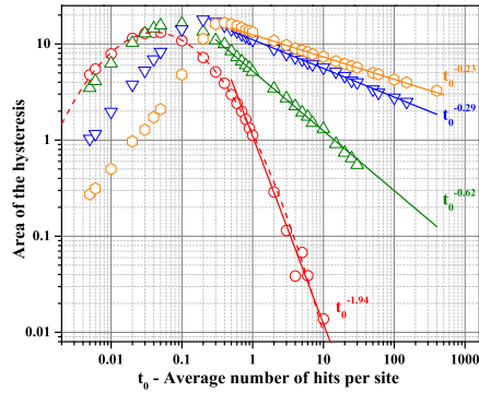
Figure 13. Effect of increasing \beta on the relative hysteresis area for \bar{a} for different holding times t_0 per stress level in a stress ramp from 0 to 25 in increments of 1 (with \alpha = 8 ). The dash line is a log-normal fit and the full lines are the fitted power laws indicated in the inserts. The symbols refer to the value of the interaction parameter \beta : circles ( \circ ) - \beta = 0 , up triangles ( \triangle ) - \beta = 1.5 , down triangles ( \nabla ) - \beta = 3 , hexagons ( \hexagon ) - \beta = 3.5 .
