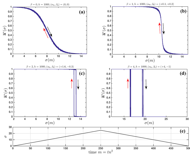
Figure 12. Results of five distinct Gibbs field simulations corresponding to an increasing/decreasing stress ramp (illustrated in the bottom panel) with \alpha = 8 and \beta \in \{0, 1, 2, 4\} indicated on the top of each panel). The stress was increased from 0 to 25 in units of 0.01 and decreased back to 0 with a holding time of h = 1000 (nearly asymptotic state for each value of the applied stress) as the site configuration varied from \mathbf{1} to \mathbf{0} and then back to \mathbf{1} . The arrows indicate the increasing/decreasing branches of the stress ramp.
