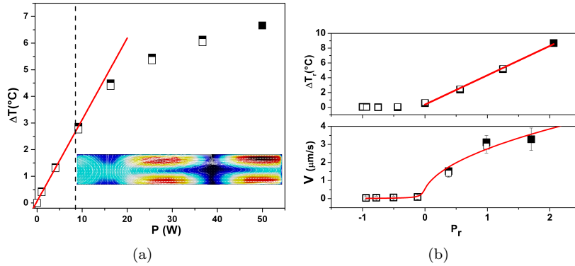
Figure 42. (a) Dependence of the temperature gradient \Delta T within Glycerin on the heat flux P . The full/empty symbols refer to increasing/decreasing heat flux. The vertical dashed line marks the transition between the conductive and convective regimes. A typical DPIV measured convection pattern is illustrated in the insert. (b) (Top) Dependence of the reduced temperature \Delta T_r on the reduced power. The line is a linear fit. (Bottom) Dependence of the pattern amplitude V on the reduced power P_r . The line is a nonlinear fit according to Landau’s theory of imperfect bifurcations, Eq. 48.
