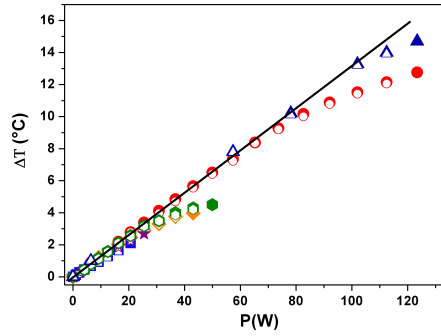
Figure 44. Dependence of temperature gradient on the heat flux for six values of the Carbopol ® concentration: ( \triangle , \blacktriangle ) - c = 0.11\%wt , ( \circ , \bullet ) - c = 0.1\%wt , ( \square , \square ) - c = 0.08\%wt , ( \diamond , \diamond ) - c = 0.075\%wt , ( \star , \star ) - c = 0.06\%wt , ( \square , \blacksquare ) - c = 0.05\%wt . The full/empty symbols refer to increasing/decreasing heat flux. The full line is a linear fit.
