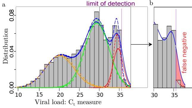
Figure 3: (a) Representation of the density for the classical mixing Gaussian model (dashed lines) and the partially censored model (solid lines) each composed as a sum of 3 components for the Gaussian model (orange/green/red dashed lines) and the partially censored model (orange/green/red solid lines); (purple vertical line) location of the threshold d_{\text{cens}} \approx 35.6 . (b) Focus on the false negative region, with the estimated false negative probability in the partially censored model (solid line) due to the defect of detection above the threshold d_{\text{cens}} (red color filled area).
