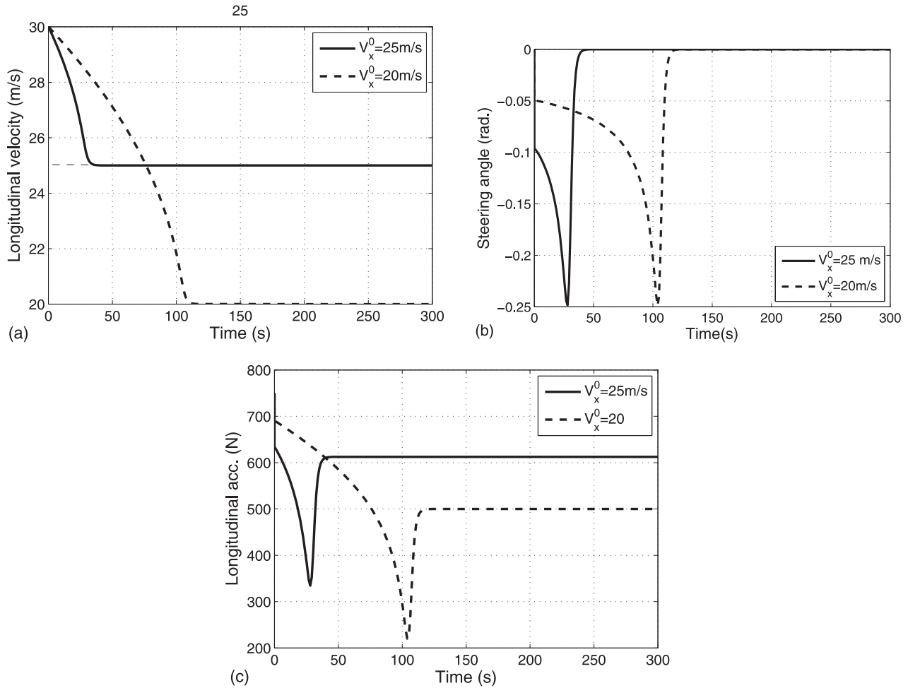
Figure 5. Stabilisation of vehicle at two desired velocities: V_x^0 = 25 and V_x^0 = 20 m/s: (a) longitudinal velocity V_x ; (b) steering angle \delta and (c) acceleration force F_1 .
