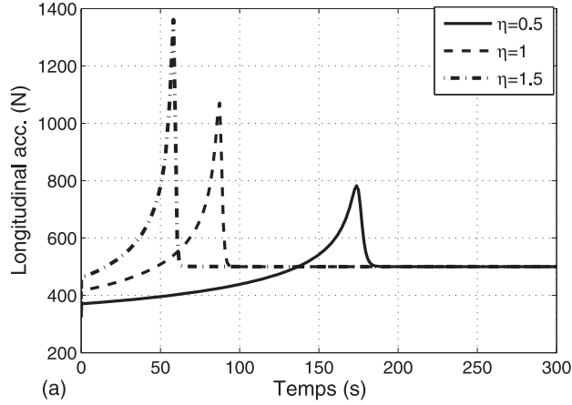
Figure 3. Acceleration and steering responses of the vehicle with different parameter \eta : (a) acceleration force input F_l and (b) steering angle input \delta .
