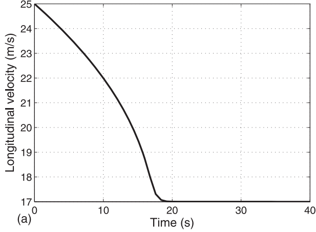
Figure 6. Stabilisation of vehicle at desired velocity V_x = 17 m/s: (a) from 25 to 17 m/s and (b) from 6 to 17 m/s.
