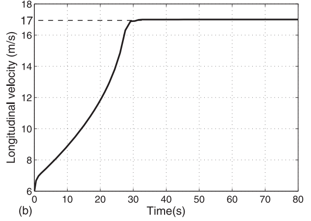
Figure 6. Stabilisation of vehicle at desired velocity V_x = 17 m/s: (a) from 25 to 17 m/s and (b) from 6 to 17 m/s.
