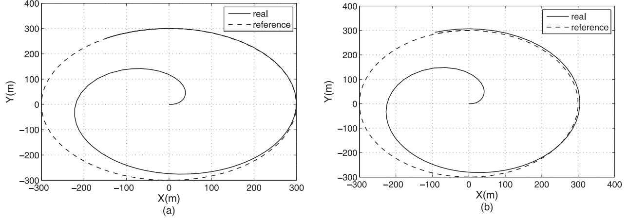
Figure 7. Vehicle trajectory tracking in XY plane: (a) with constant parameters \alpha = 0.014 and \beta = 0.01 and (b) constant parameters \alpha = 0.02 and \beta = 0.015 .
