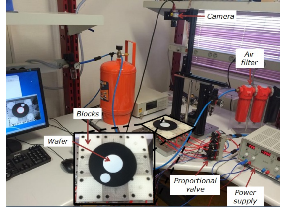
Fig. 10. Setup of the closed-loop experiments.
