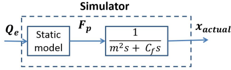
Fig. 6. Simulator block diagram.
