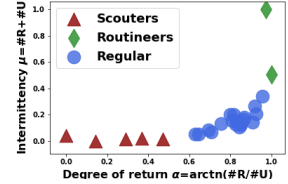
Figure 4: Macaco
