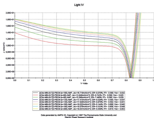
Fig. 5 Simulation by AMPS-1D of the characteristics J(V) of the organic solar cell based on [(Cbz-Mth)-B-T]2-PCBM for different thicknesses.
