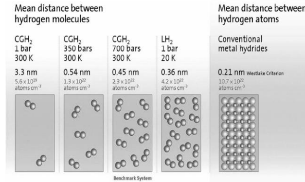
Fig. 4. Hydrogen density according the storage medium [4] [5].
