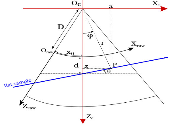
Fig. 4. 2D acquisition model.
