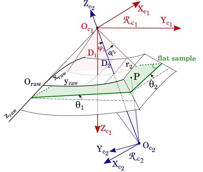
Fig. 6. 3D acquisition scheme when taking into account the convex and concave forms of the deformation.
