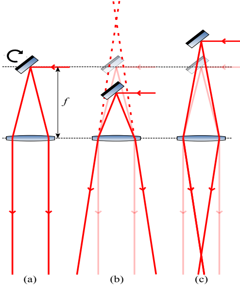
Fig. 3. Illustration of the source of image distortions: (a) the focal point is on the mirror, there is no distortion, (b) the focal point is behind the mirror, the image distortion is convex, (c) the focal point is in front of the mirror, the image distortion is concave.
