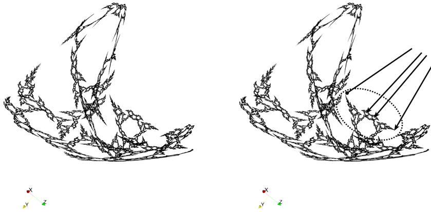
Figure 7: The representation m023-1 is of type (3, 3, 6).
