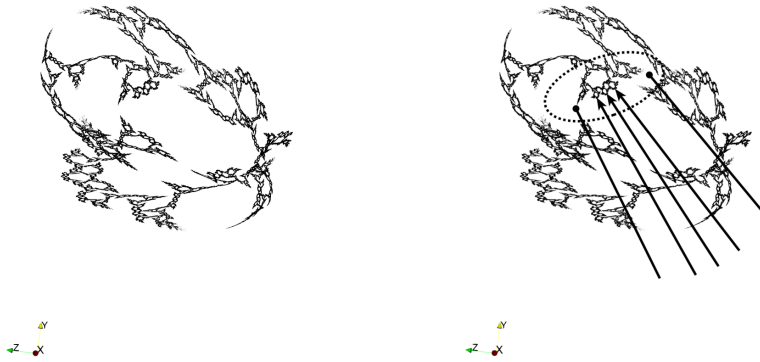
Figure 8: The representation m032-7 is of type (3, 3, 7).
