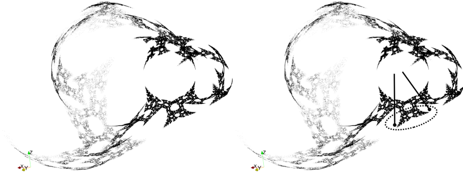
Figure 5: The representation m022-1 is of type (3, 3, 4) .
