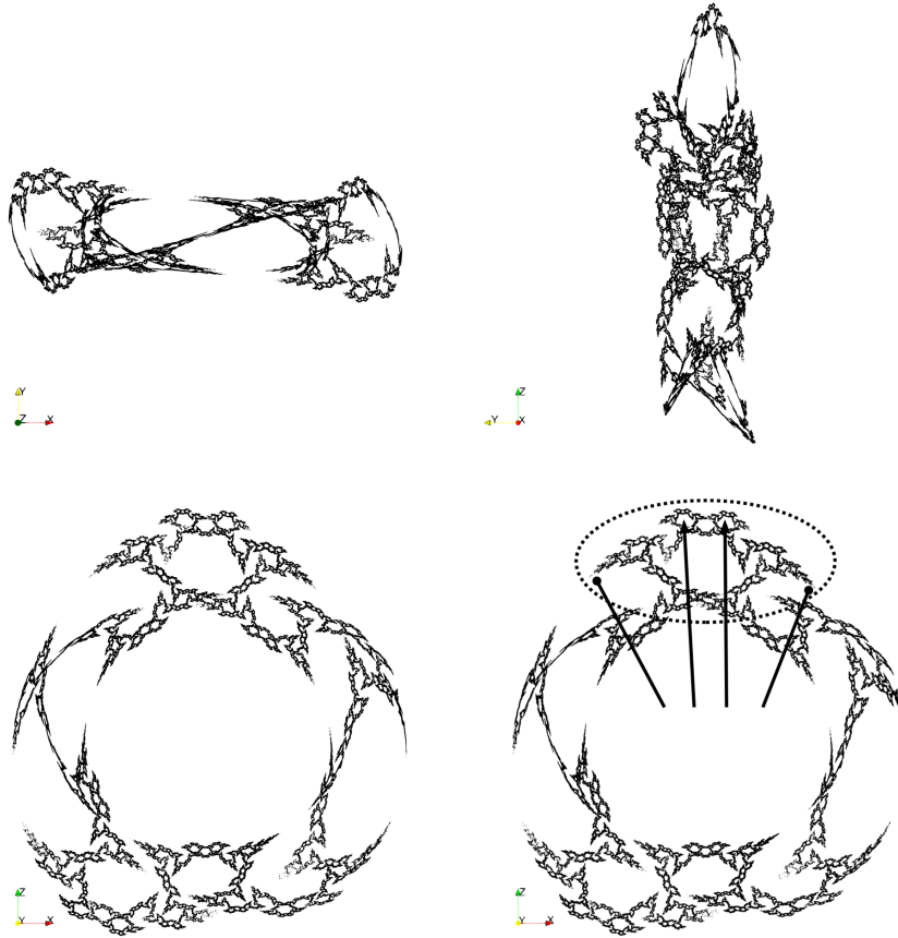
Figure 3: Hyperbolic triangle group (3,3,6) with I_2I_3I_1I_3 parabolic.
