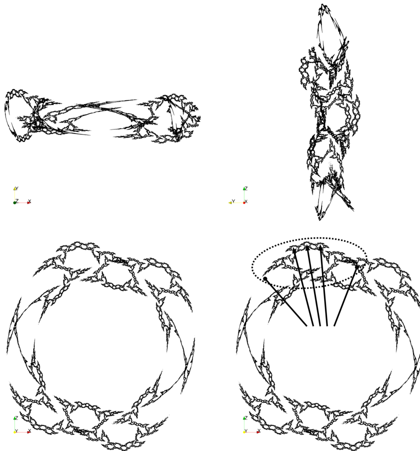
Figure 4: Hyperbolic triangle group (3, 3, 7) with I_2 I_3 I_1 I_3 parabolic.
