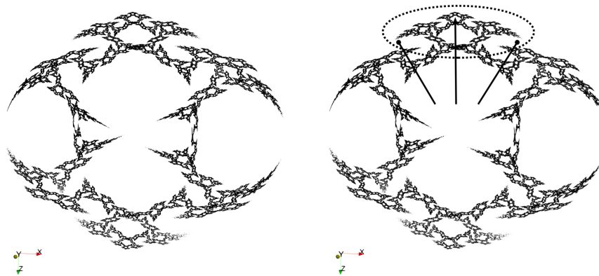
Figure 6: The representation m015-2 is of type (3, 3, 5) .
