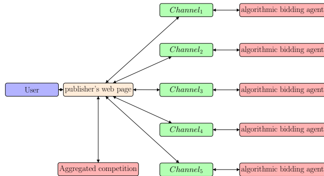
Figure 1: A user reaching a page triggers a chain of calls that end up in the buyer’s servers. At bidding time, the bidding agent might not know that other bidding agents of the same buyer are bidding for the same opportunity. Hence, his bid will be facing not only the aggregated competition, but also the bids of his fellow bidding agents. Moreover, if the agent cannot tell apart Channel_1 from Channel_2 , then its bidding strategy is bound to be the same on those two channels.
