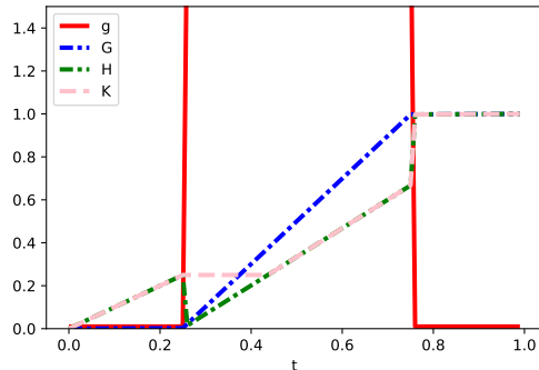
Figure 2: It is easy to build a distribution g (in red) so that the condition on H for Theorem 1 is not met. Indeed, in this example H cannot be a cumulative distribution (not monotone). However, the solution identified in Theorem 1 can be adapted (see discussion in the text).
