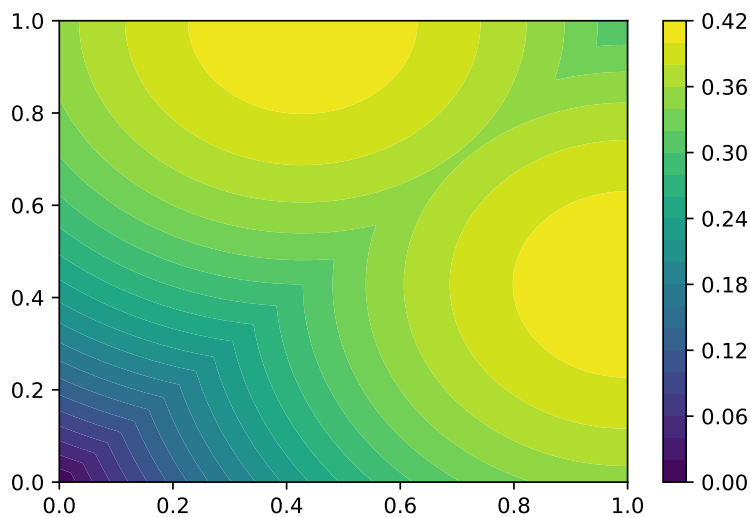
Figure 4: Here we suppose that we can define channel specific strategies. The expected payoff as a function of the bids on channel 1 and channel 2. We set the probability of being called by only one channel equal to 0.3 each, and the probability to be called by both at the same time equal to 0.4 and the competition is uniform on [0,1] and v = 1 . We note that even in this simple situation, the expected payoff is not convex. This illustrates the fact that finding an optimal shading strategy might be complicated in practice.
