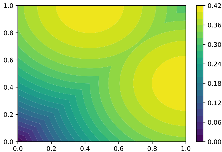
Figure 4: Here we suppose that we can define channel specific strategies. The expected payoff as a function of the bids on channel 1 and channel 2. We set the probability of being called by only one channel equal to 0.3 each, and the probability to be called by both at the same time equal to 0.4 and the competition is uniform on [0,1] and v = 1 . We note that even in this simple situation, the expected payoff is not convex. This illustrates the fact that finding an optimal shading strategy might be complicated in practice.
