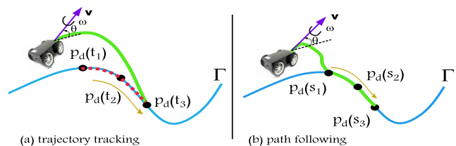
Fig. 1. Trajectory tracking versus path following.
