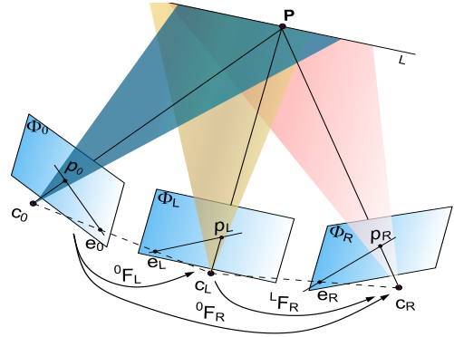
Fig. 4. The three-view geometry.
