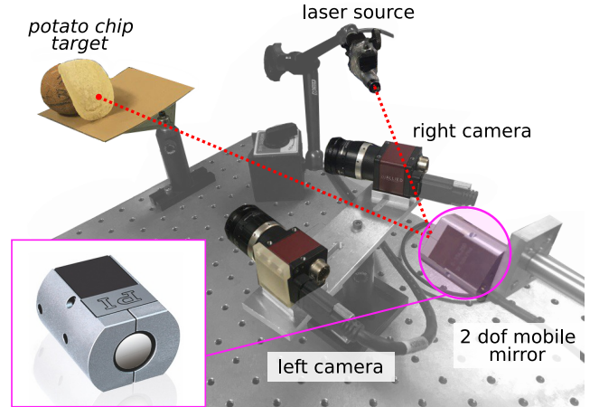
Fig. 13. Photography of the experimental set-up.
