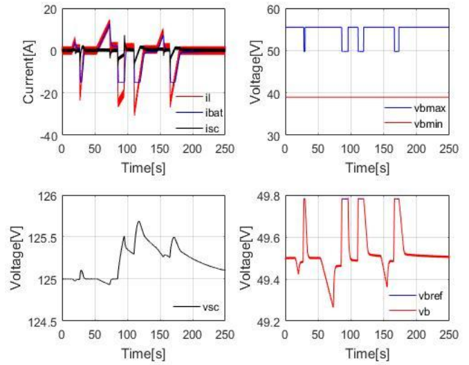
Fig. 5. Simulation results in charge mode
