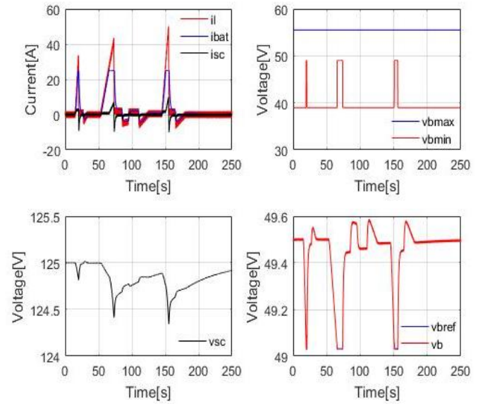
Fig. 6. Simulation results in discharge mode
