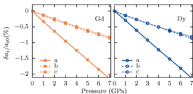
Figure 5 Compressibility of the unit-cell parameters [( a i - a 0 )/ a 0 ] of GdMn 2 O 5 and DyMn 2 O 5 with respect to their ambient-pressure values, a 0 , calculated by DFT.
